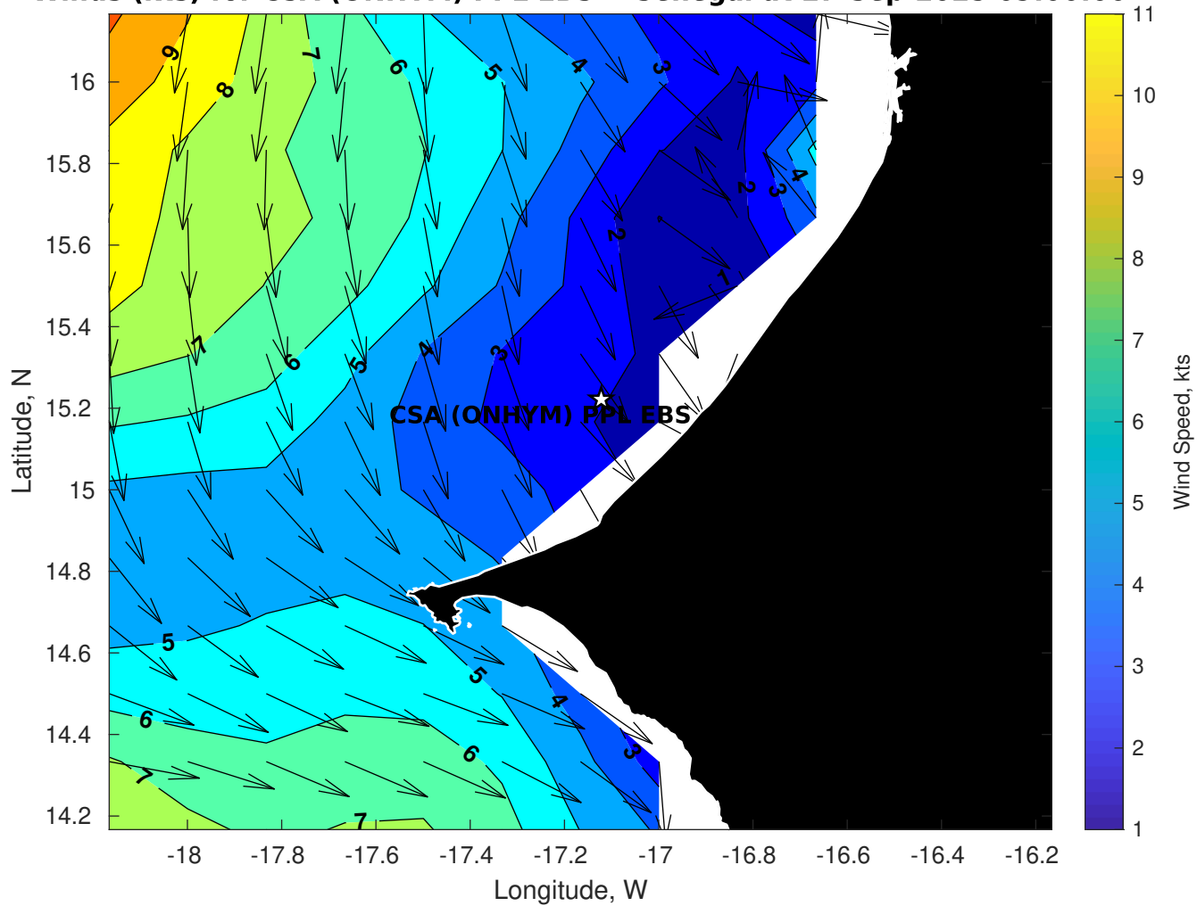
Winds (kts) for CSA (ONHYM) PPL EBS - Senegal at 27-Sep-2025 09:00:00
