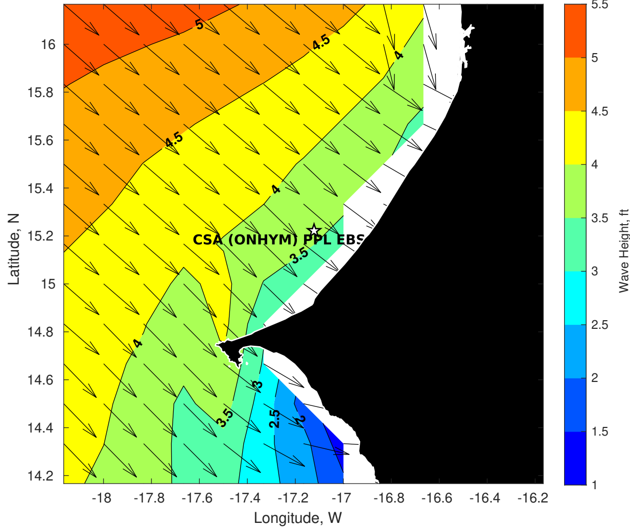
Wave Height (ft) for CSA (ONHYM) PPL EBS - Senegal at 27-Sep-2025 09:00:00
