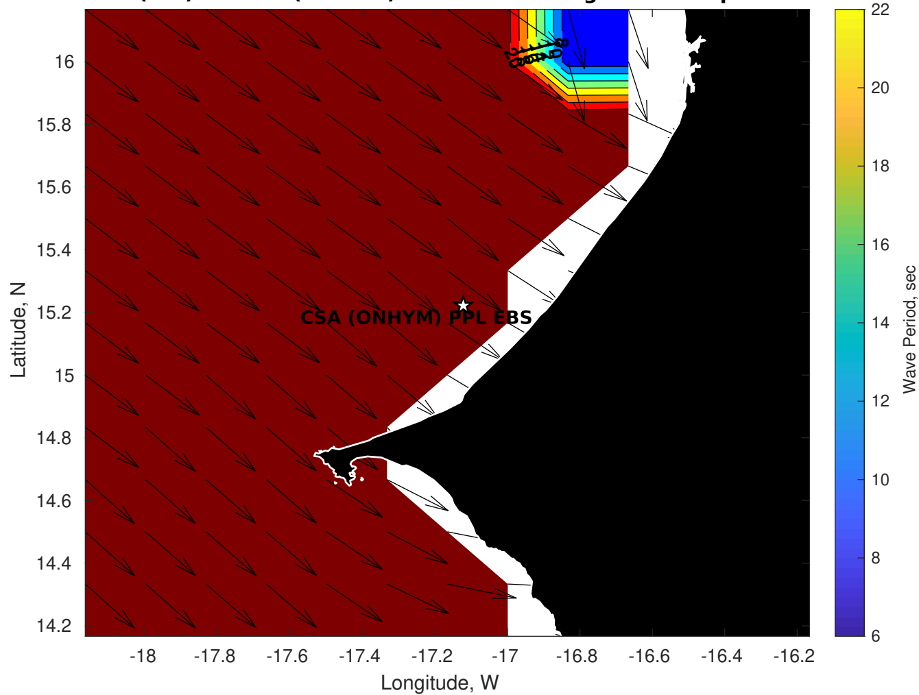
Wave Period (sec) for CSA (ONHYM) PPL EBS - Senegal at 27-Sep-2025 09:00:00
