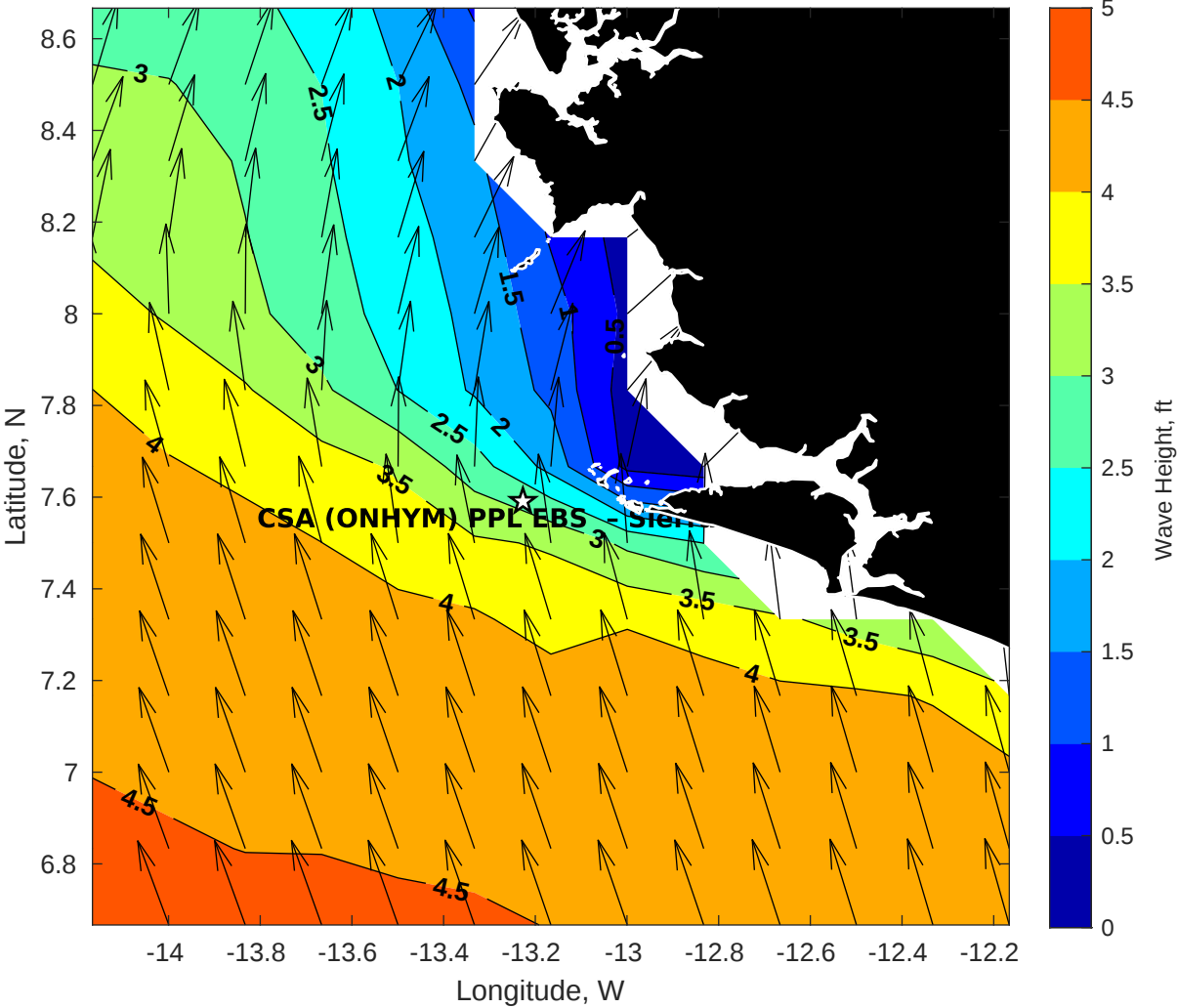
Wave Height (ft) for CSA (ONHYM) PPL EBS - Sierra Leone at 27-Sep-2025 09:00:00
