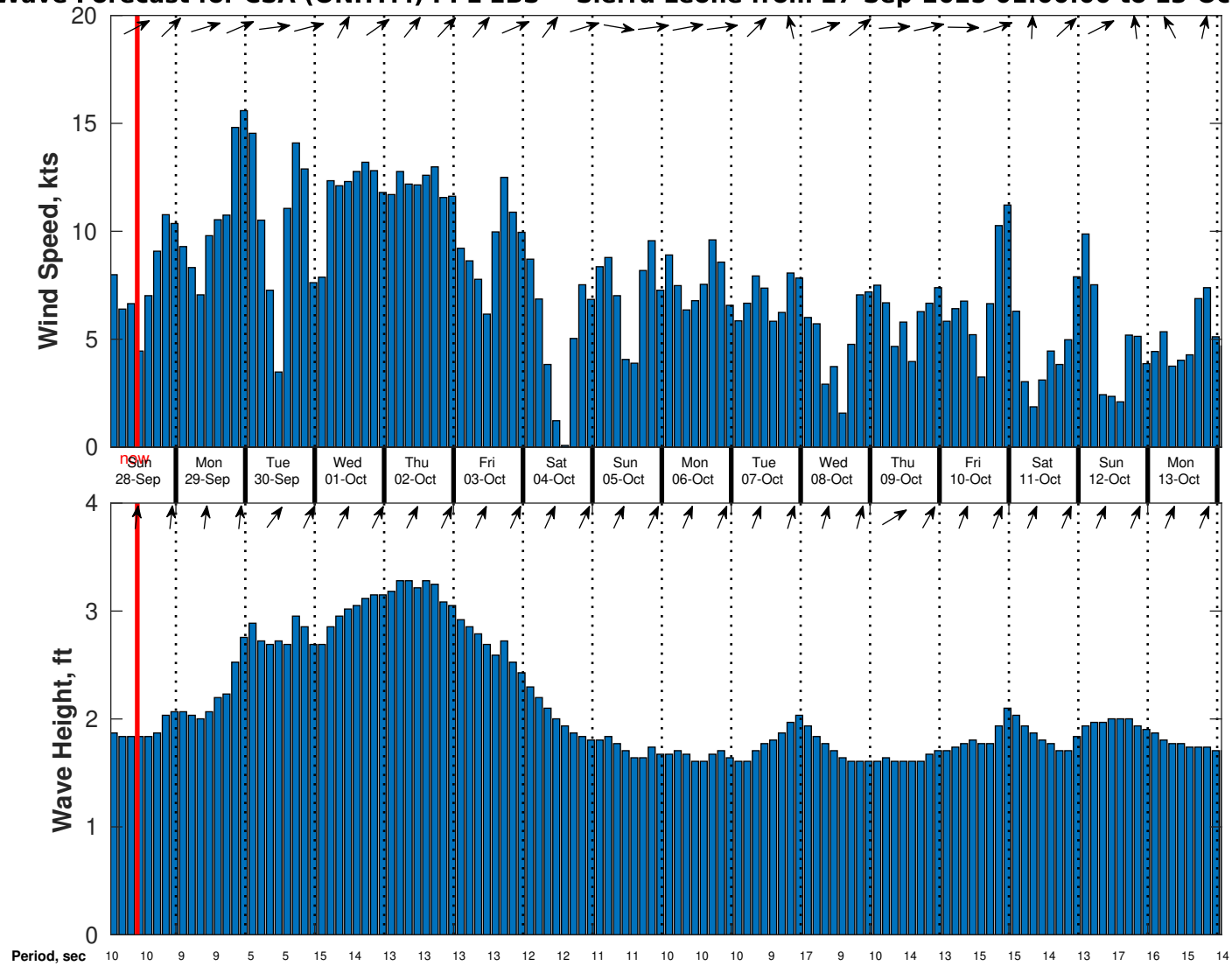
Wind & Wave Forecast for CSA (ONHYM) PPL EBS - Sierra Leone from 27-Sep-2025 01:00:00 to 13-Oct-2025 01:00:00
