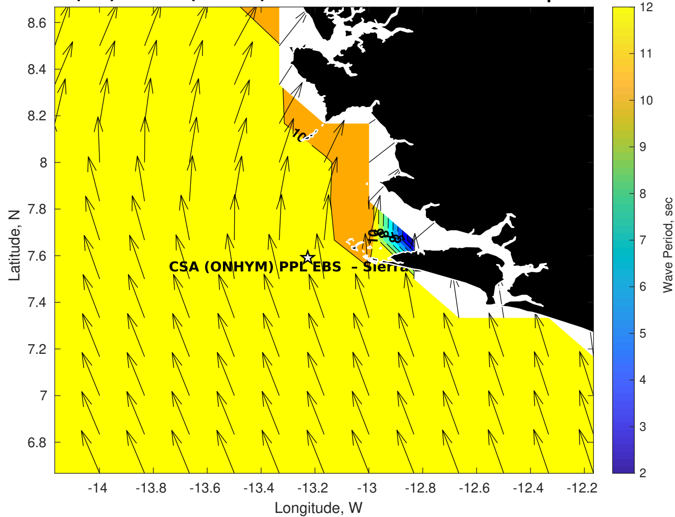
Wave Period (sec) for CSA (ONHYM) PPL EBS - Sierra Leone at 27-Sep-2025 09:00:00
