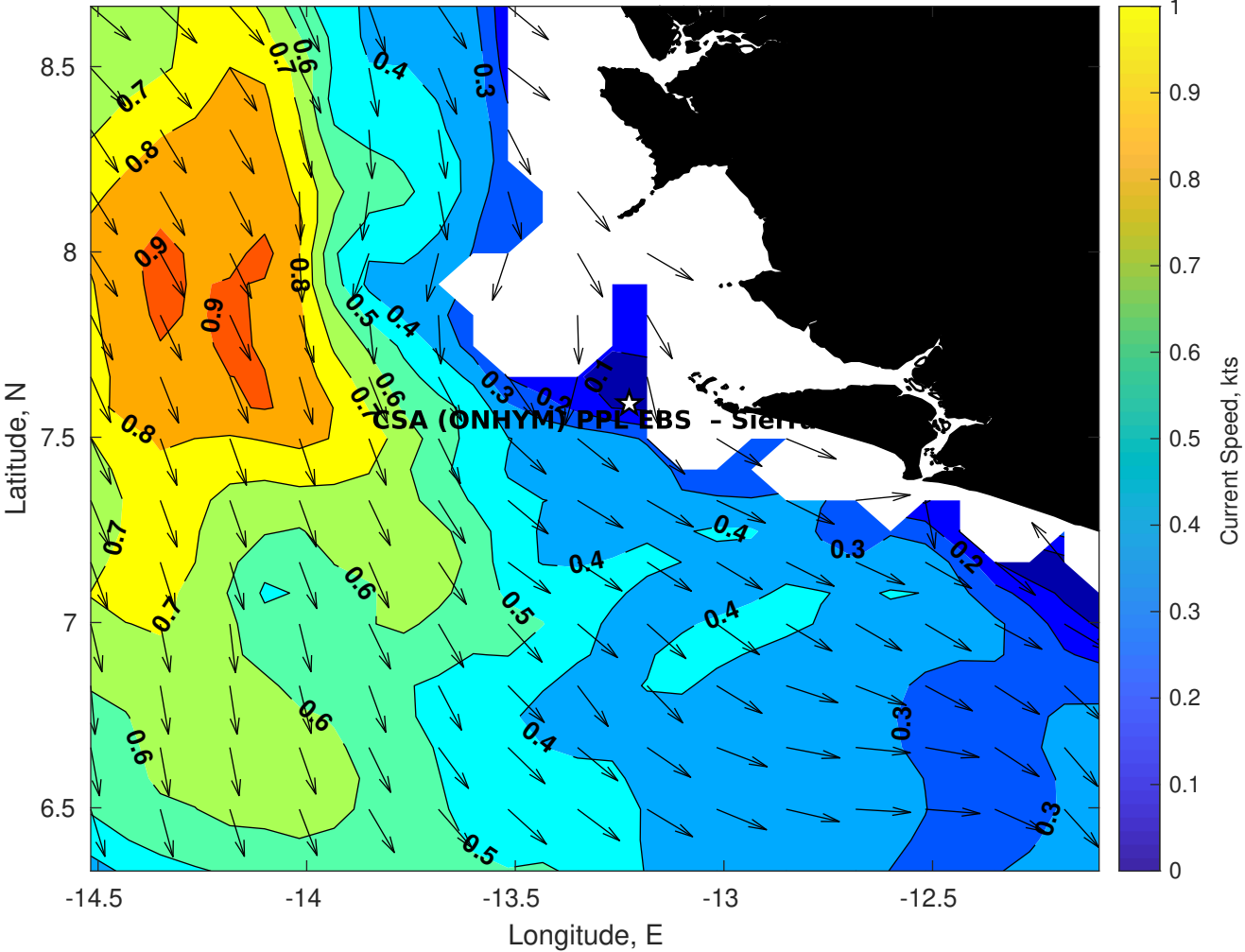
Surface Currents for CSA (ONHYM) PPL EBS - Sierra Leone at 17-Sep-2025 00:00:00
