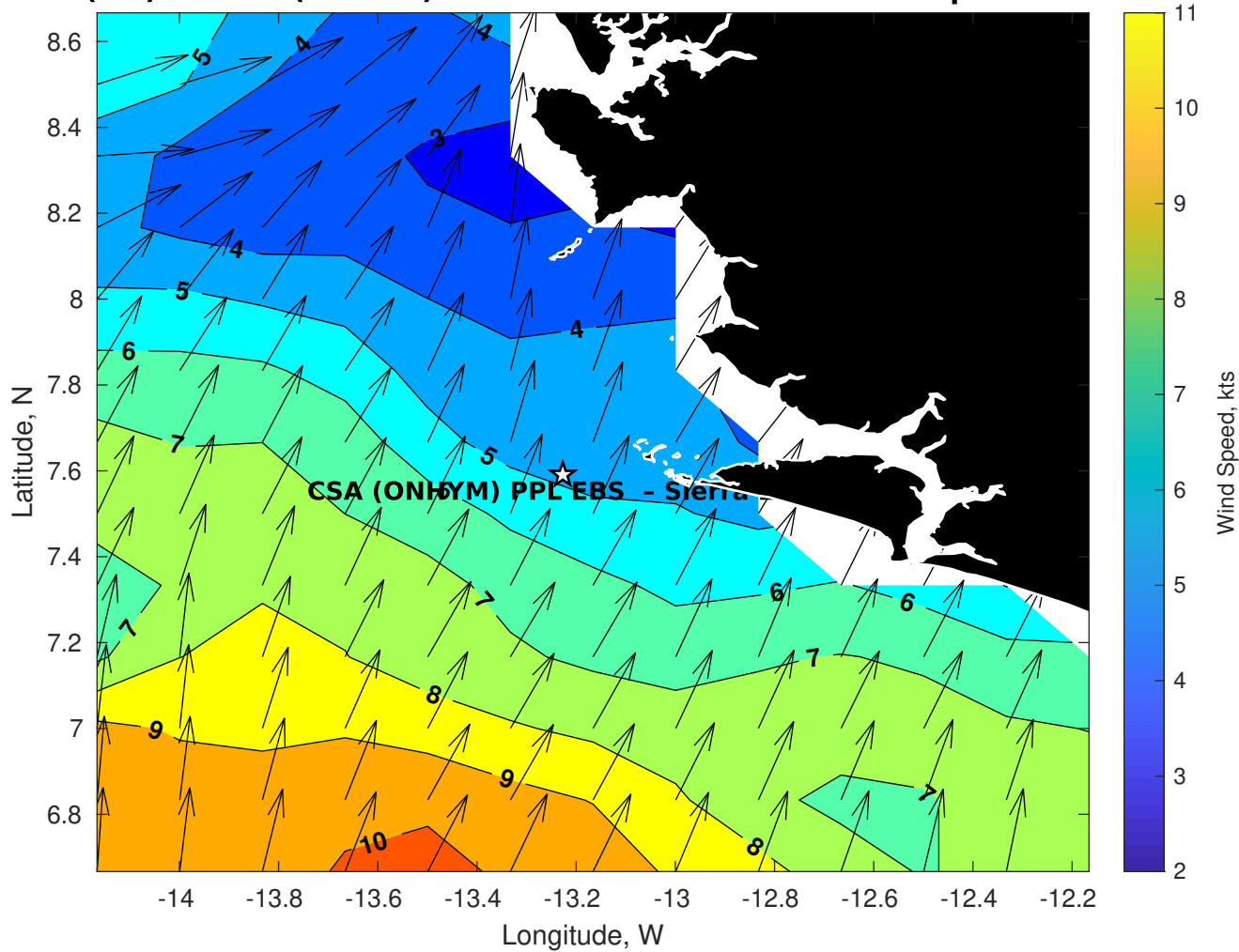
Winds (kts) for CSA (ONHYM) PPL EBS - Sierra Leone at 27-Sep-2025 09:00:00
