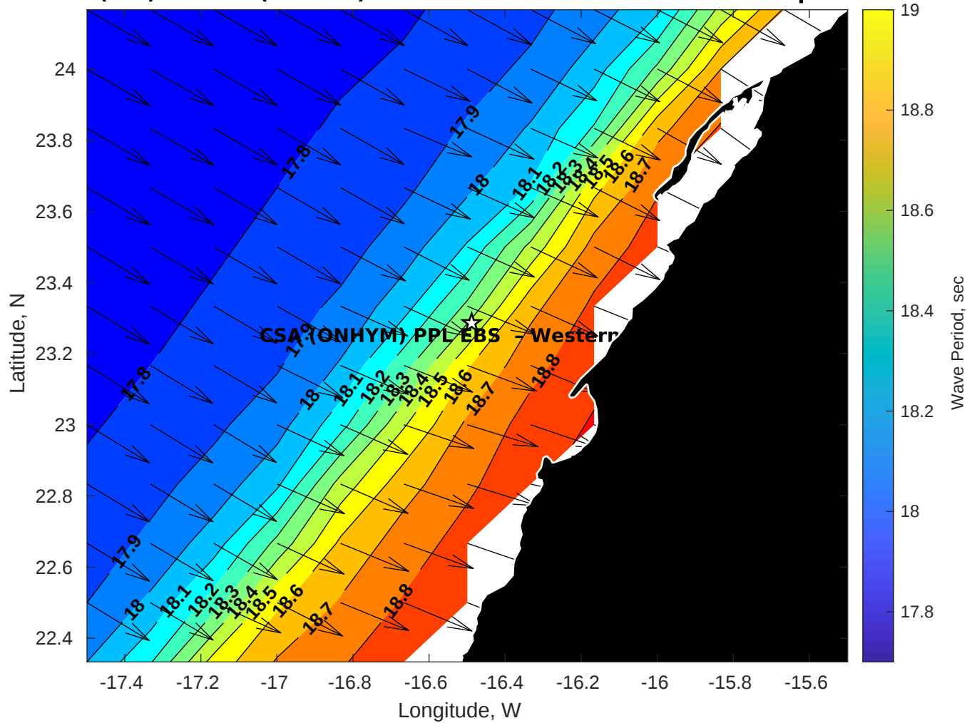
Wave Period (sec) for CSA (ONHYM) PPL EBS - Western Sahara at 27-Sep-2025 09:00:00
