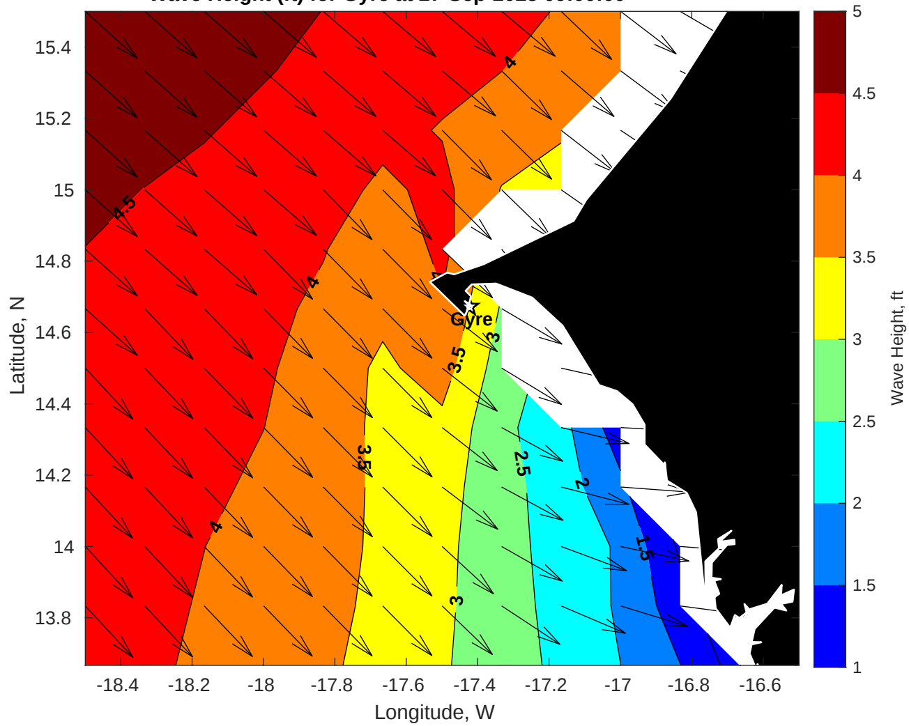
Wave Height (ft) for Gyre at 27-Sep-2025 09:00:00
