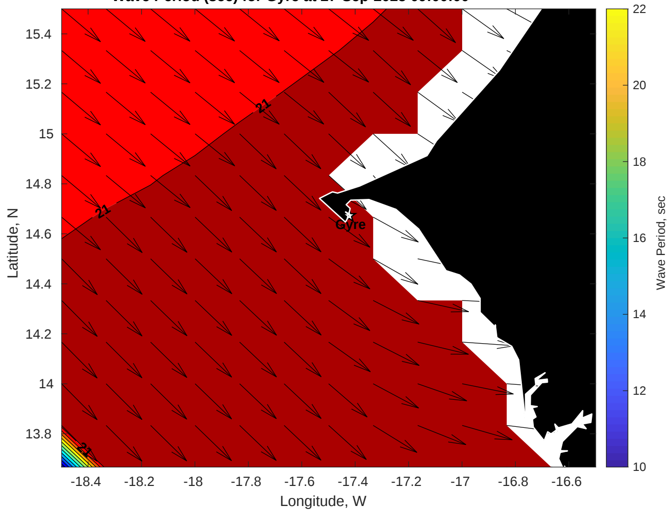
Wave Period (sec) for Gyre at 27-Sep-2025 09:00:00
