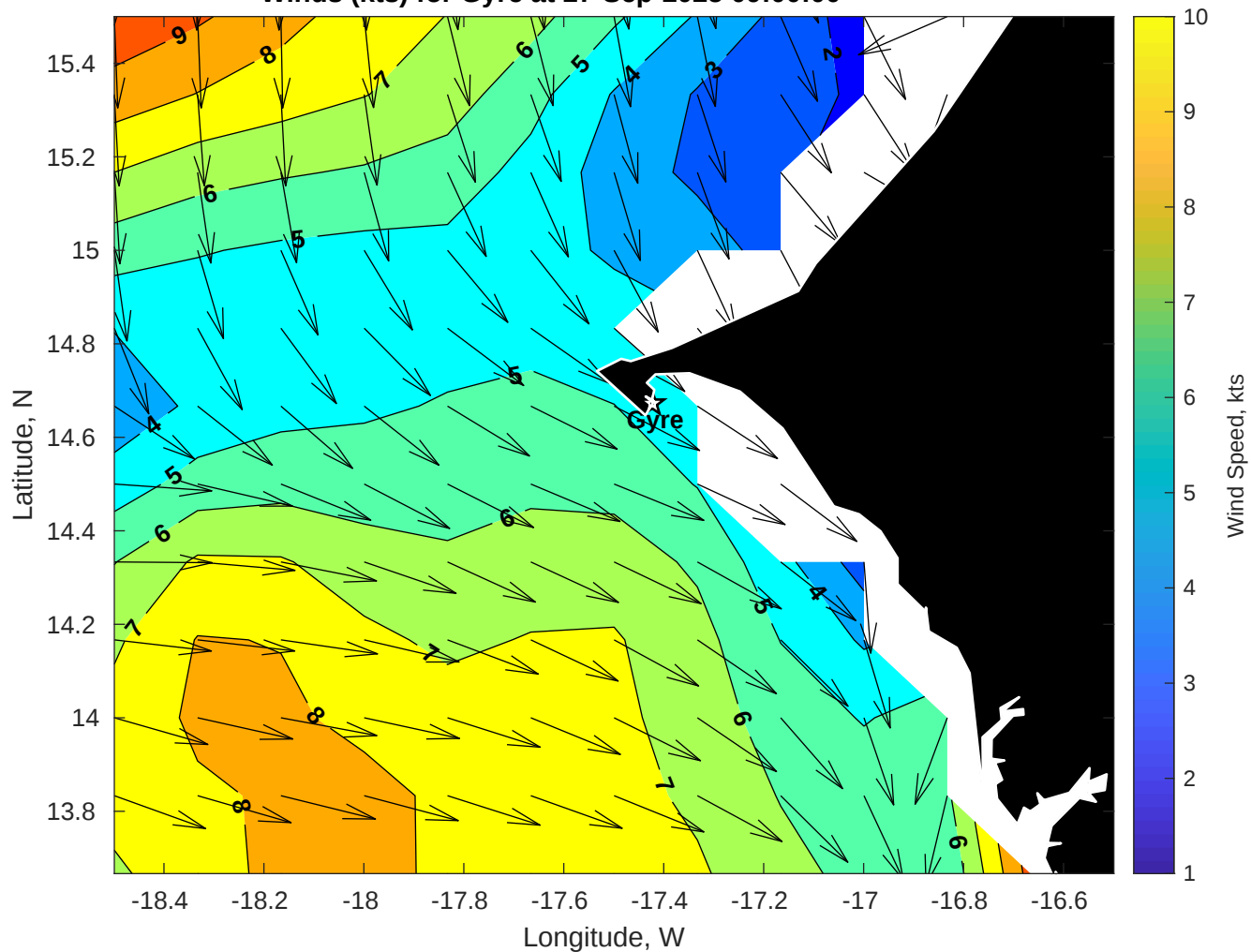
Winds (kts) for Gyre at 27-Sep-2025 09:00:00
