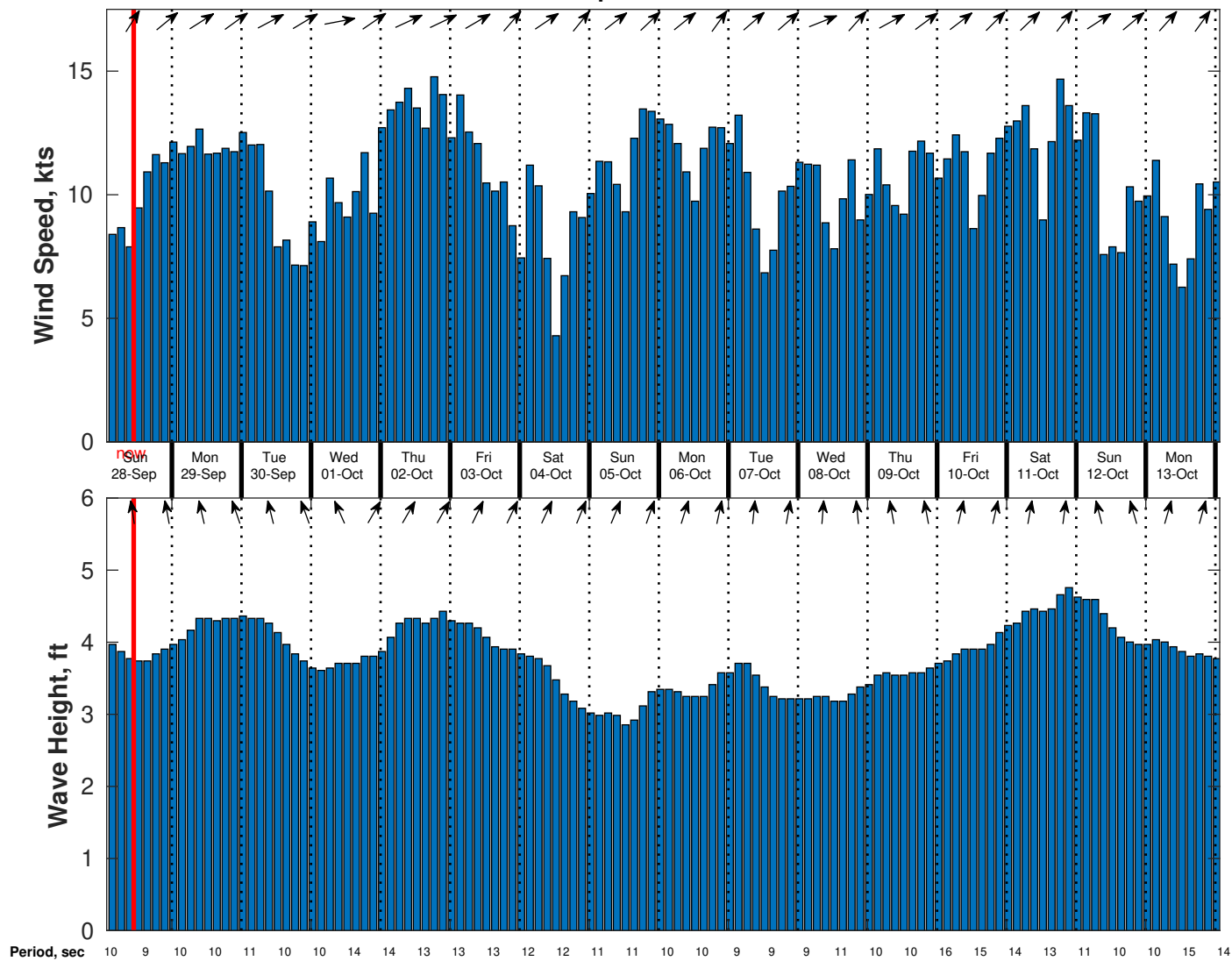
Wind & Wave Forecast for Nautilus from 27-Sep-2025 02:00:00 to 13-Oct-2025 02:00:00
