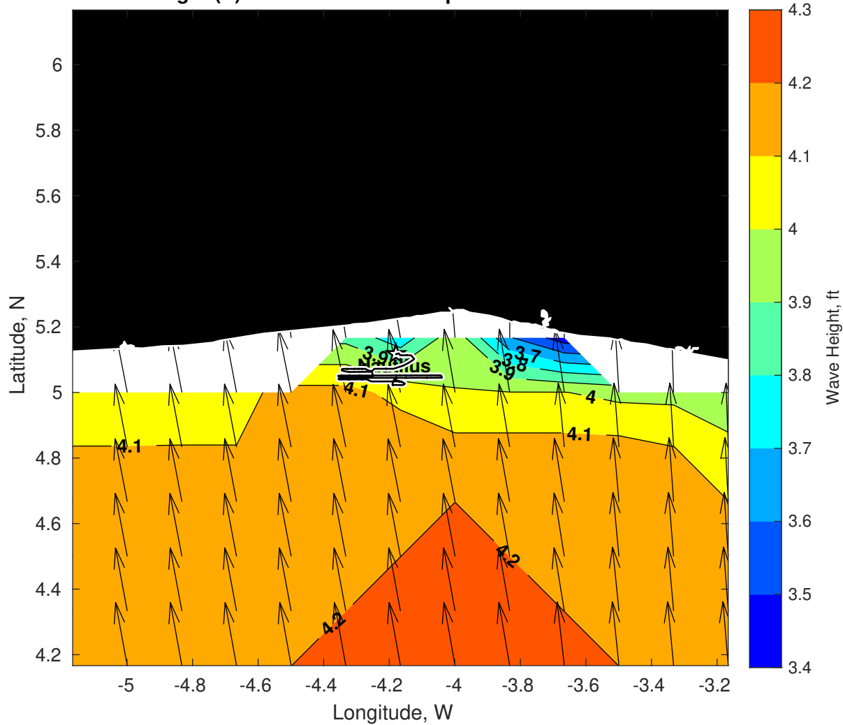
Wave Height (ft) for Nautilus at 27-Sep-2025 09:00:00
