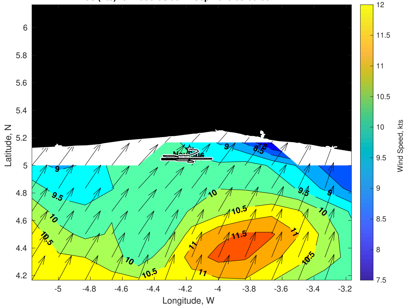
Winds (kts) for Nautilus at 27-Sep-2025 09:00:00
