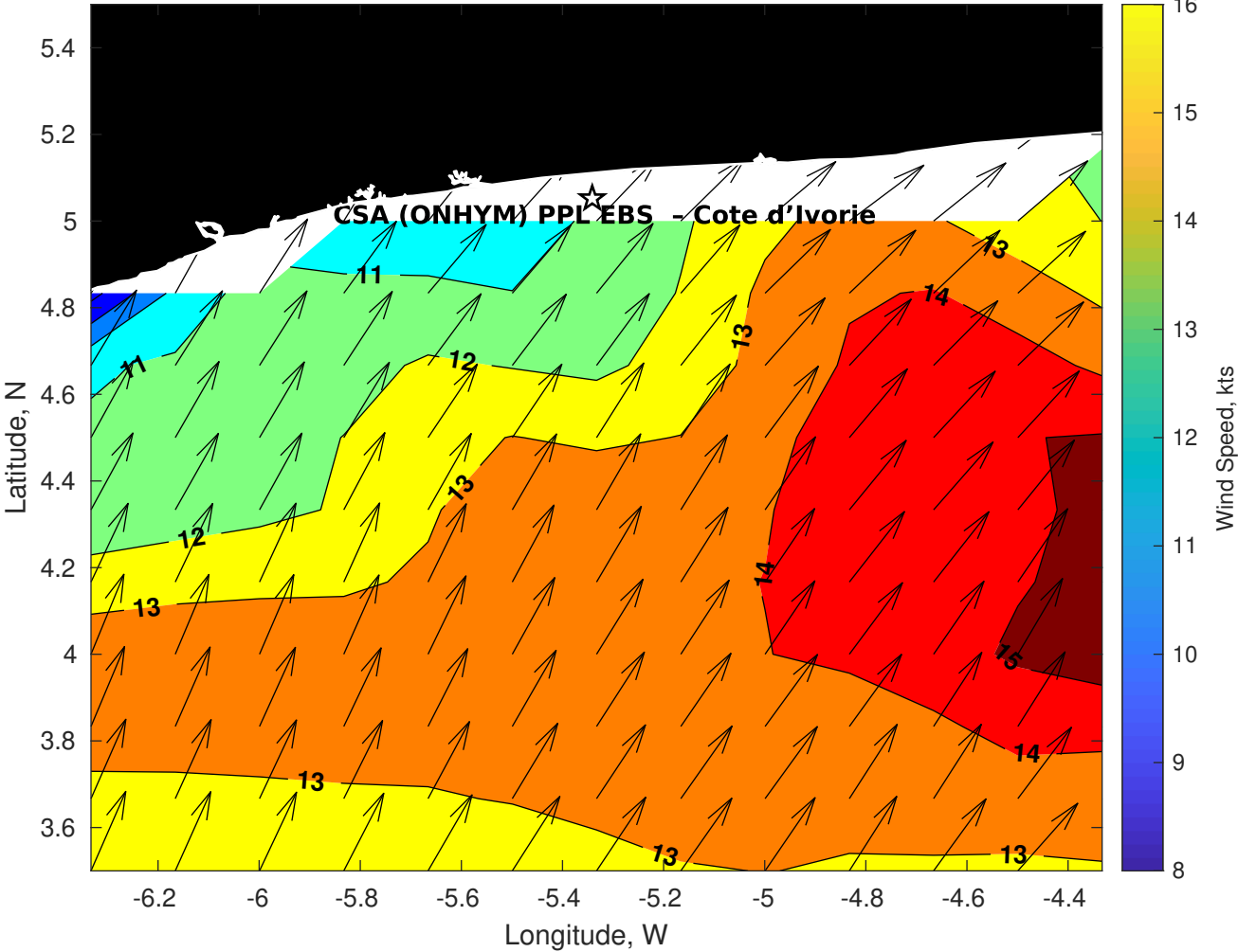
Winds (kts) for CSA (ONHYM) PPL EBS - Cote d'Ivoire at 28-Sep-2025 09:00:00
