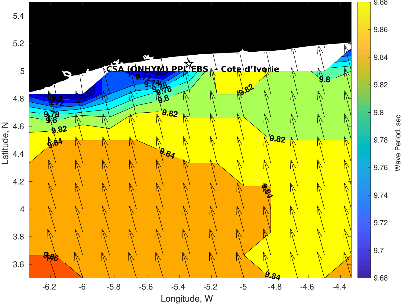
Wave Period (sec) for CSA (ONHYM) PPL EBS - Cote d'Ivoire at 28-Sep-2025 09:00:00
