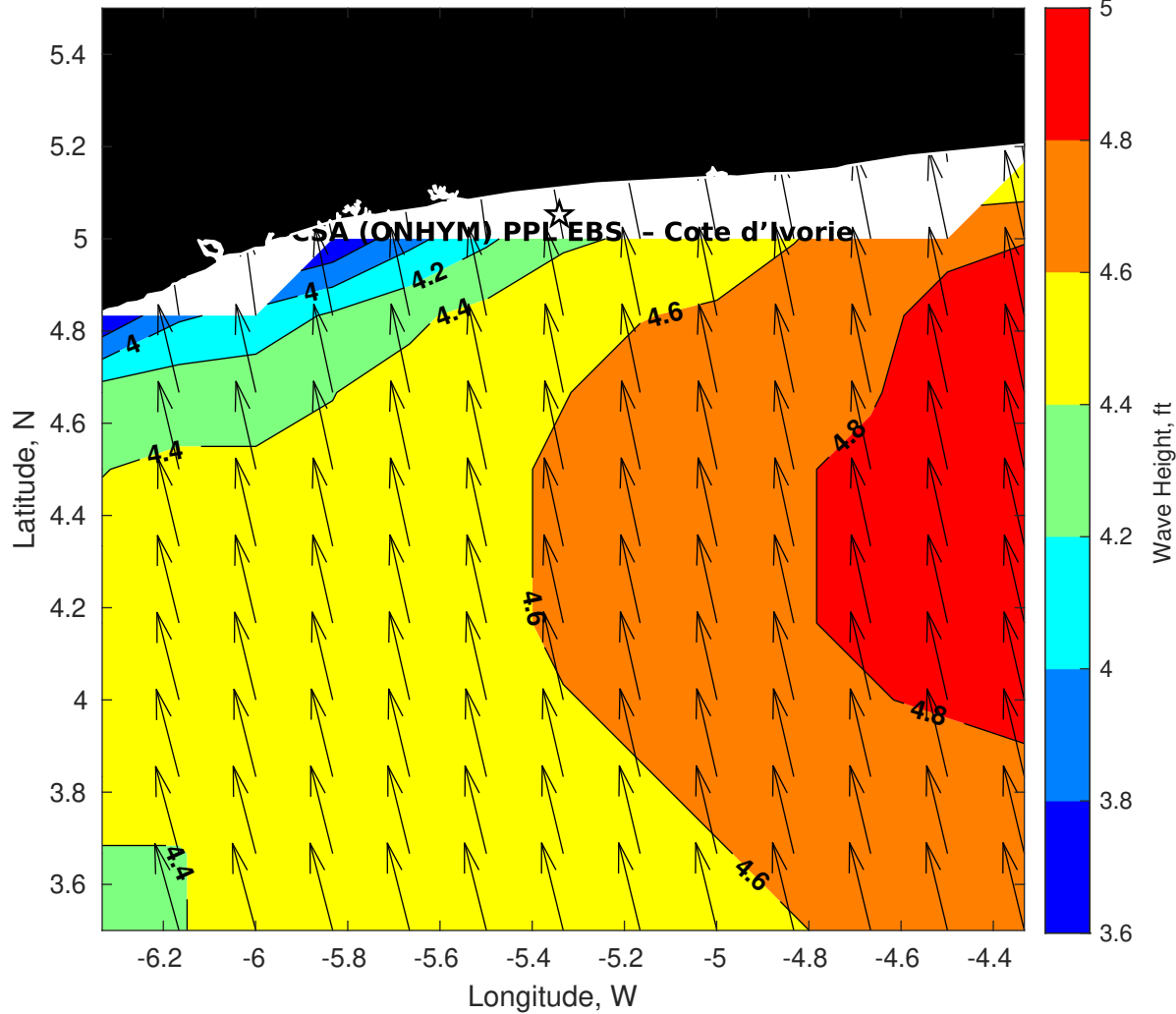
Wave Height (ft) for CSA (ONHYM) PPL EBS - Cote d'Ivoire at 28-Sep-2025 09:00:00
