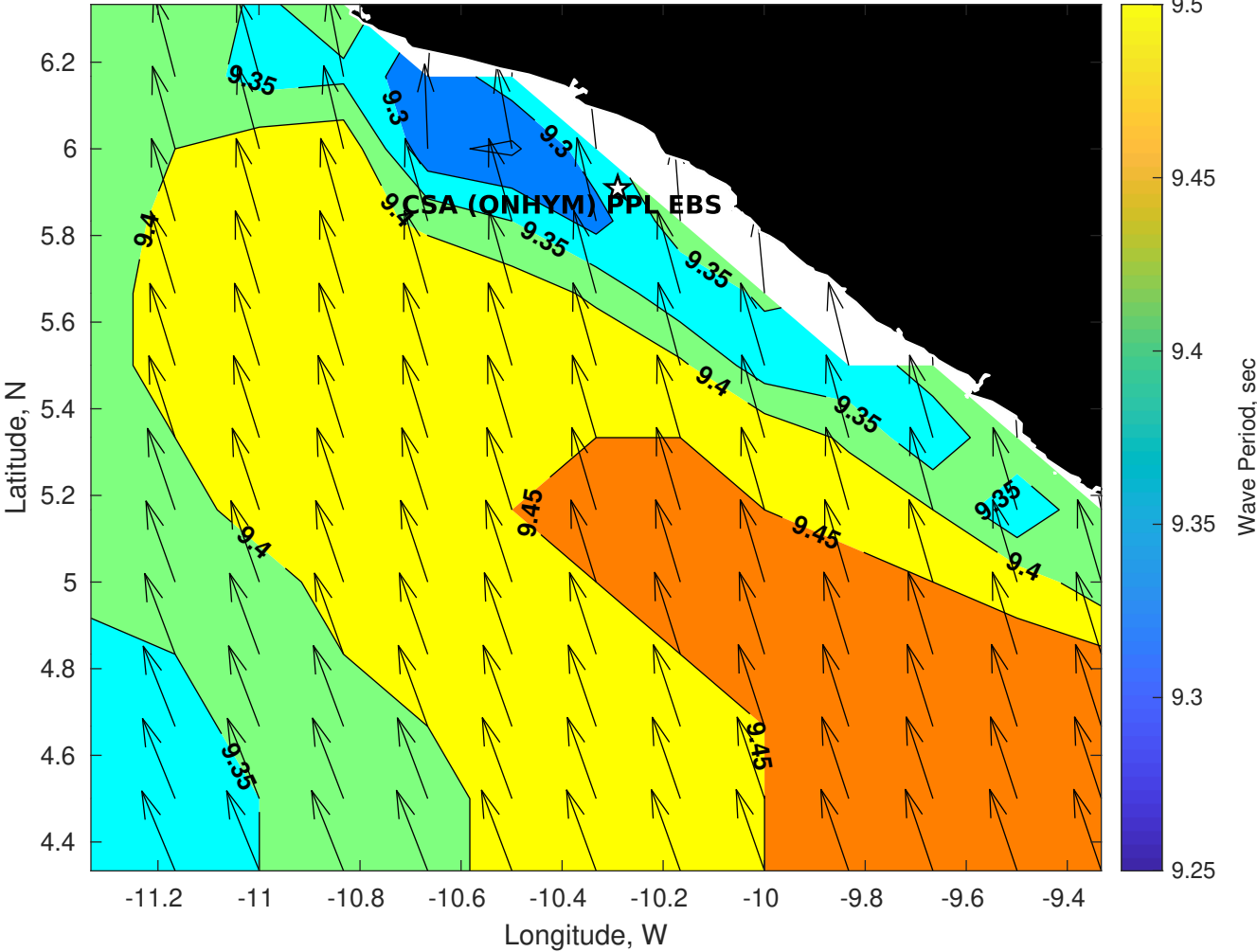
Wave Period (sec) for CSA (ONHYM) PPL EBS - Liberia at 28-Sep-2025 09:00:00
