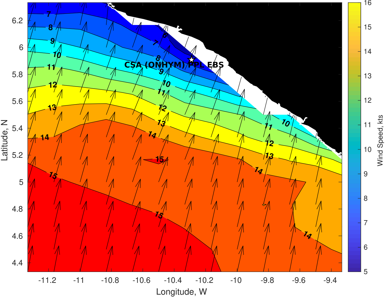
Winds (kts) for CSA (ONHYM) PPL EBS - Liberia at 28-Sep-2025 09:00:00
