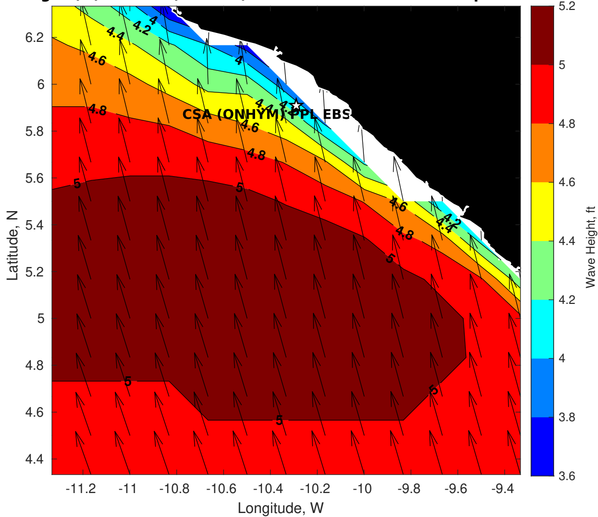
Wave Height (ft) for CSA (ONHYM) PPL EBS - Liberia at 28-Sep-2025 09:00:00
