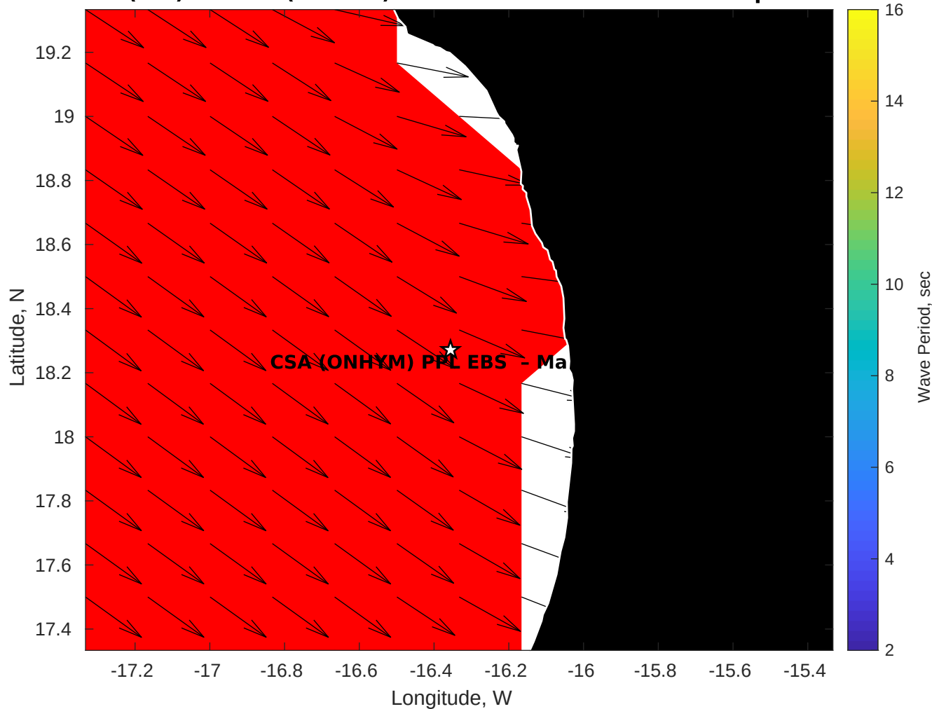
Wave Period (sec) for CSA (ONHYM) PPL EBS - Mauritania at 28-Sep-2025 09:00:00
