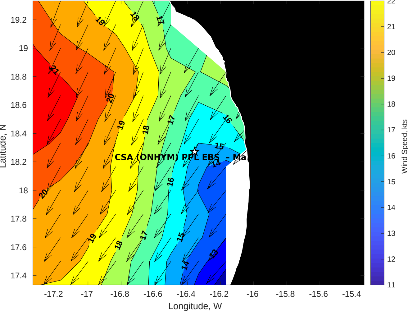
Winds (kts) for CSA (ONHYM) PPL EBS - Mauritania at 28-Sep-2025 09:00:00
