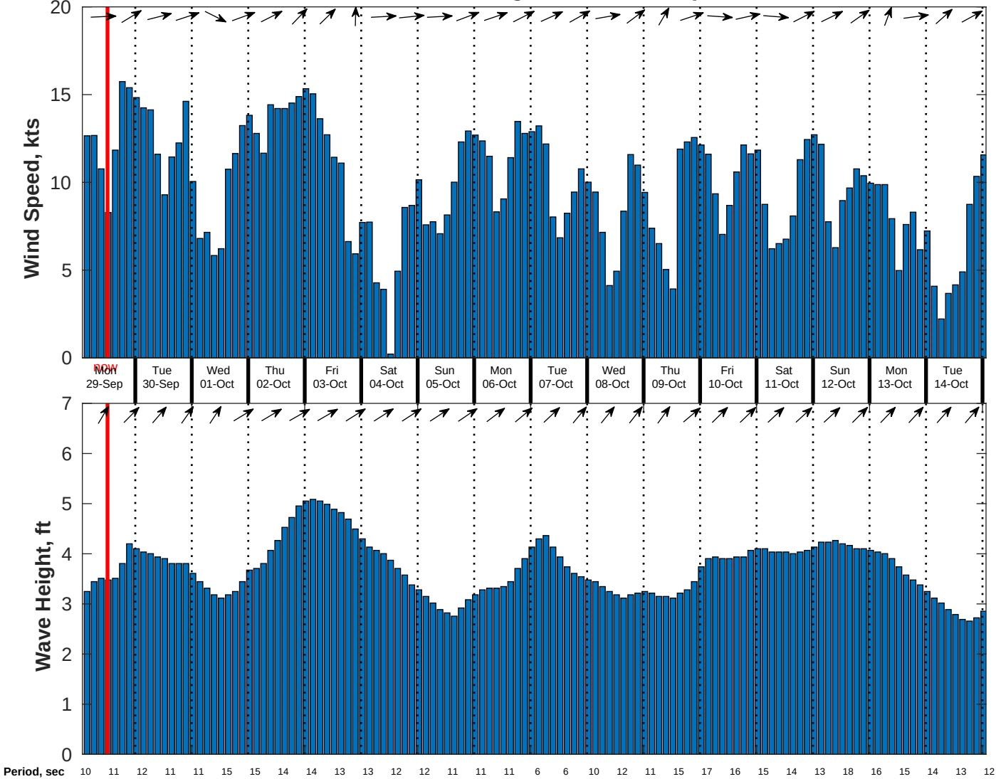
Wind & Wave Forecast for CSA (ONHYM) PPL EBS - Nigeria from 28-Sep-2025 02:00:00 to 14-Oct-2025 02:00:00
