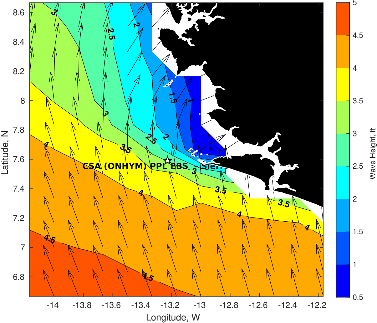
Wave Height (ft) for CSA (ONHYM) PPL EBS - Sierra Leone at 28-Sep-2025 09:00:00
