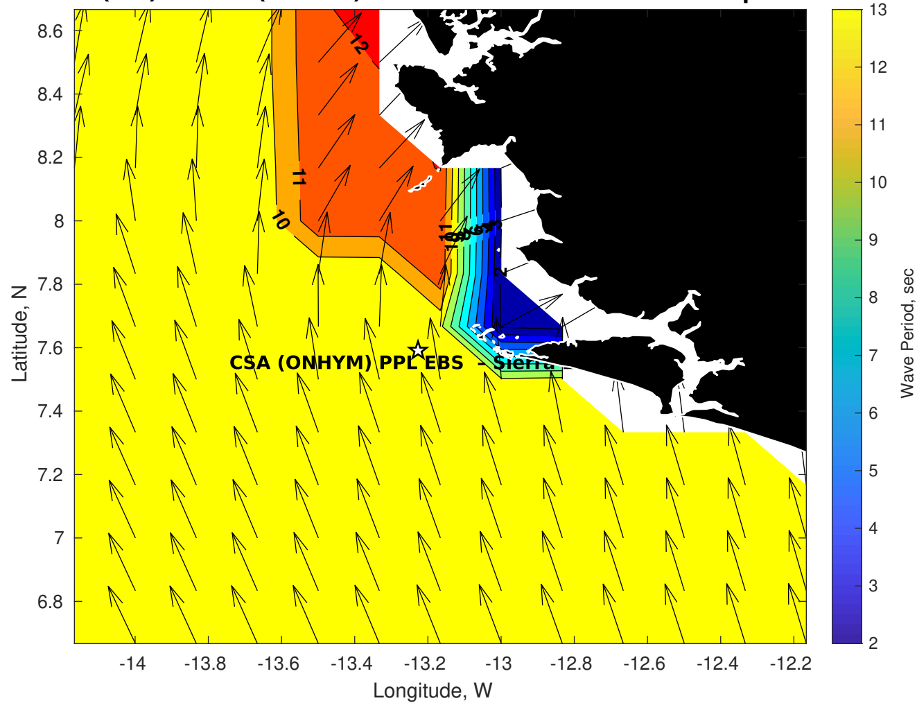
Wave Period (sec) for CSA (ONHYM) PPL EBS - Sierra Leone at 28-Sep-2025 09:00:00
