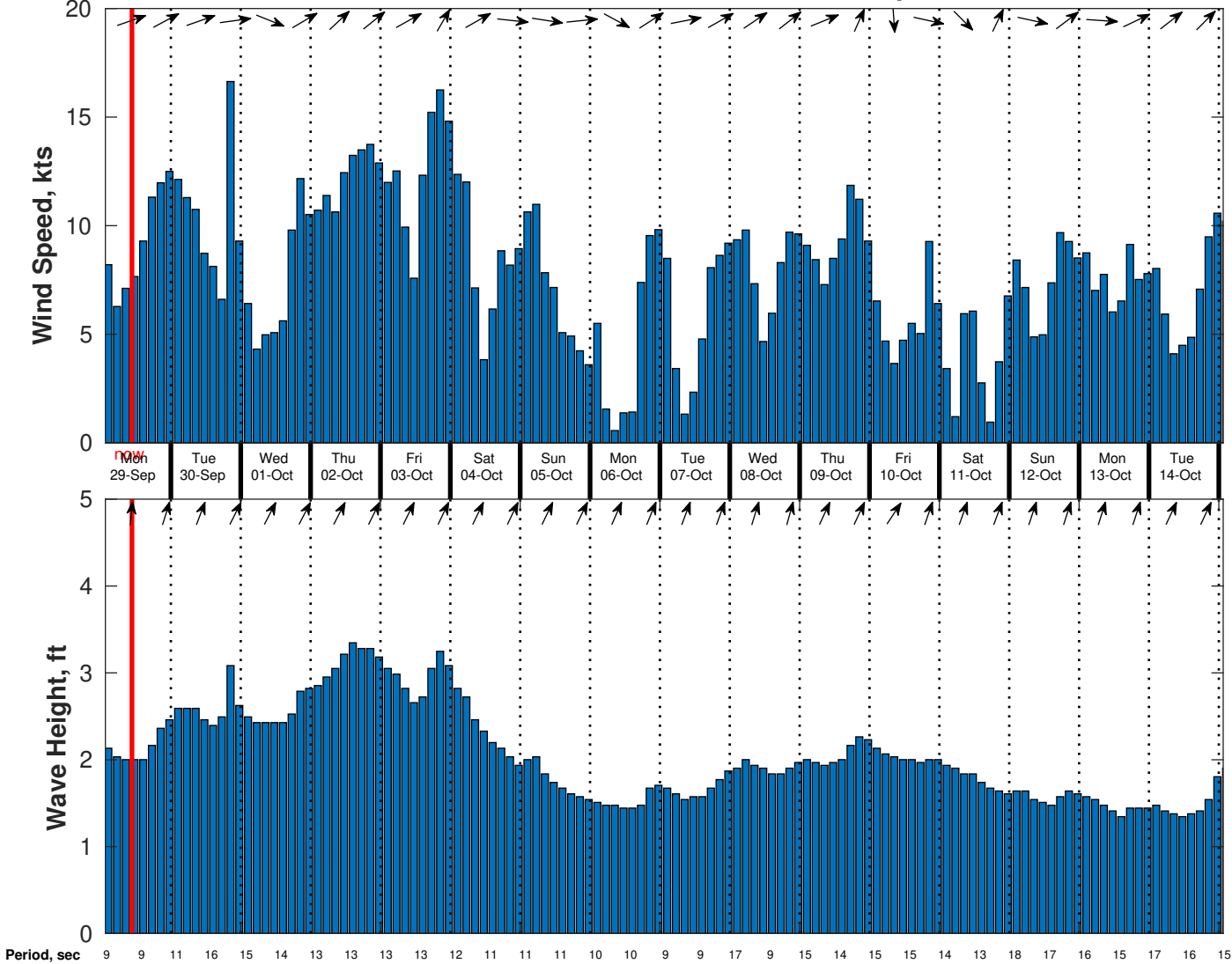
Wind & Wave Forecast for CSA (ONHYM) PPL EBS - Sierra Leone from 28-Sep-2025 01:00:00 to 14-Oct-2025 01:00:00
