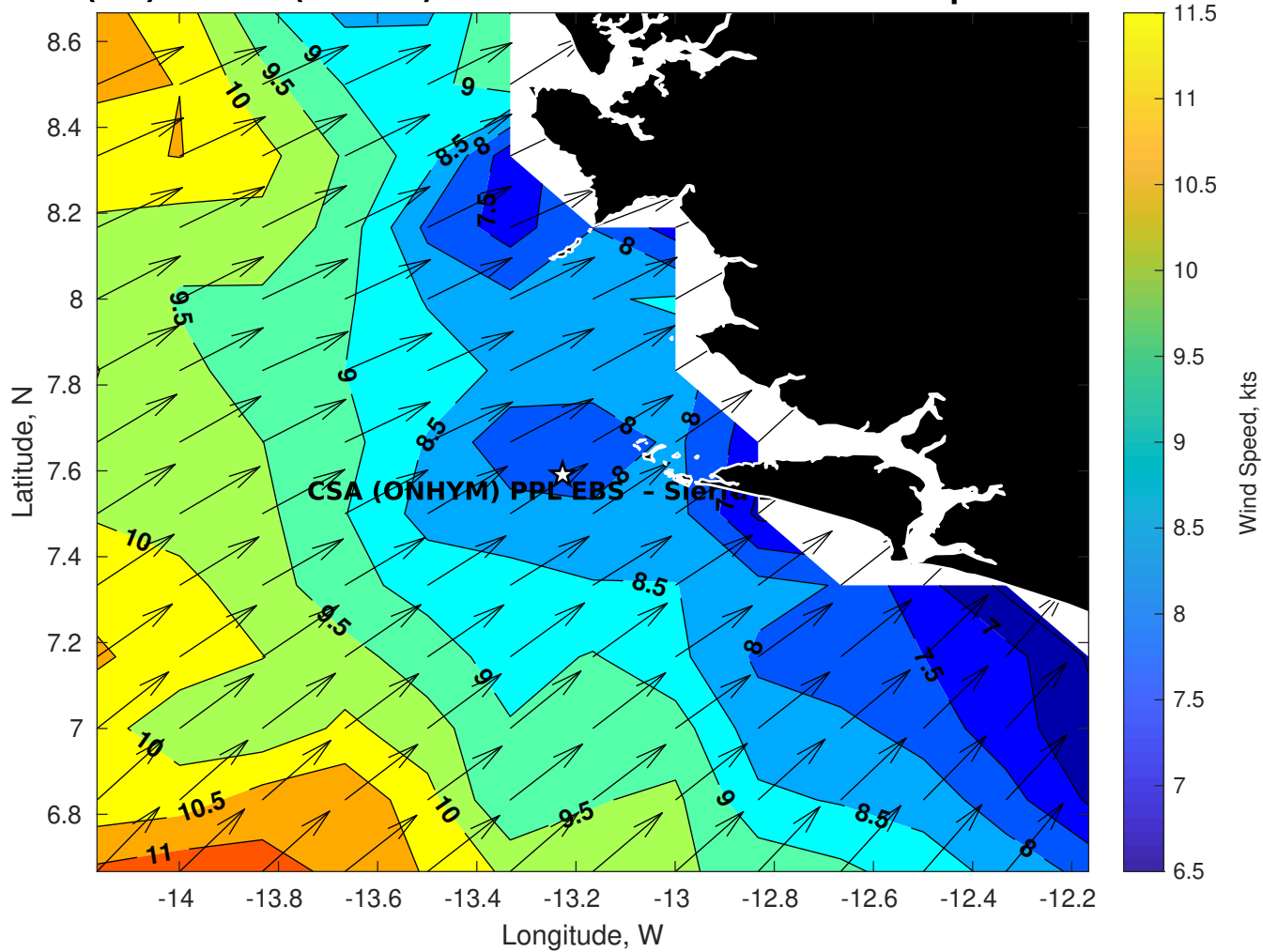
Winds (kts) for CSA (ONHYM) PPL EBS - Sierra Leone at 28-Sep-2025 09:00:00
