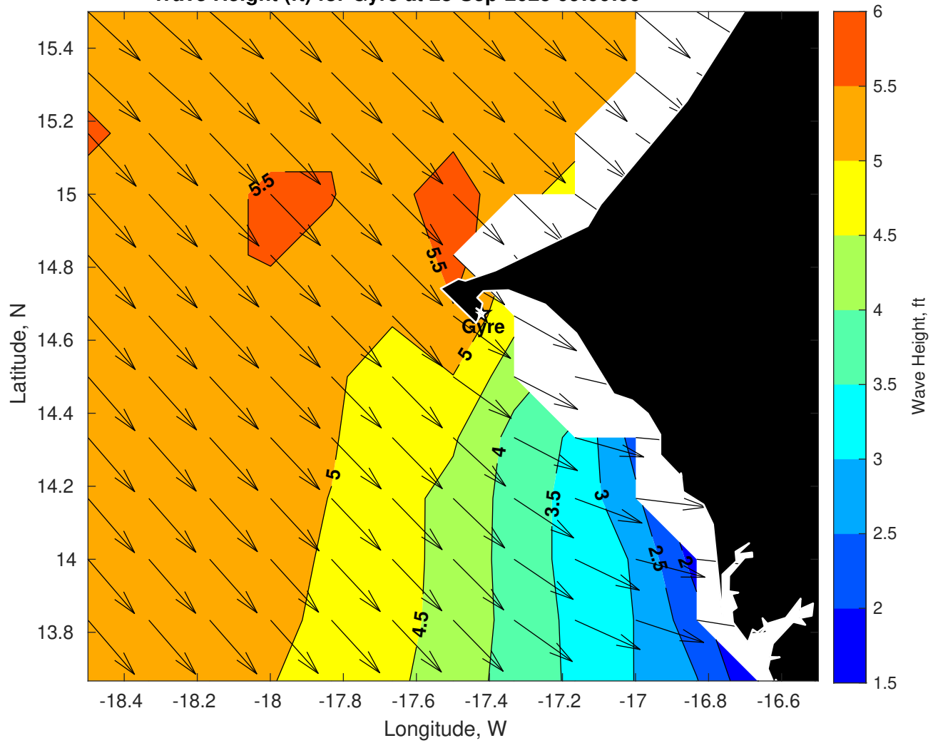
Wave Height (ft) for Gyre at 28-Sep-2025 09:00:00
