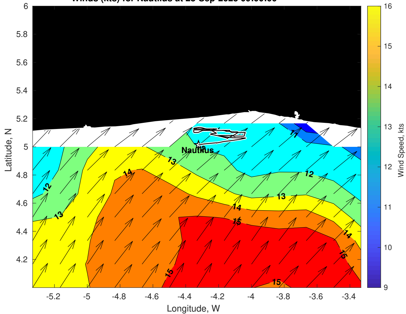
Winds (kts) for Nautilus at 28-Sep-2025 09:00:00
