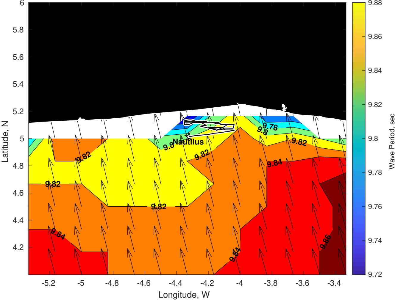
Wave Period (sec) for Nautilus at 28-Sep-2025 09:00:00
