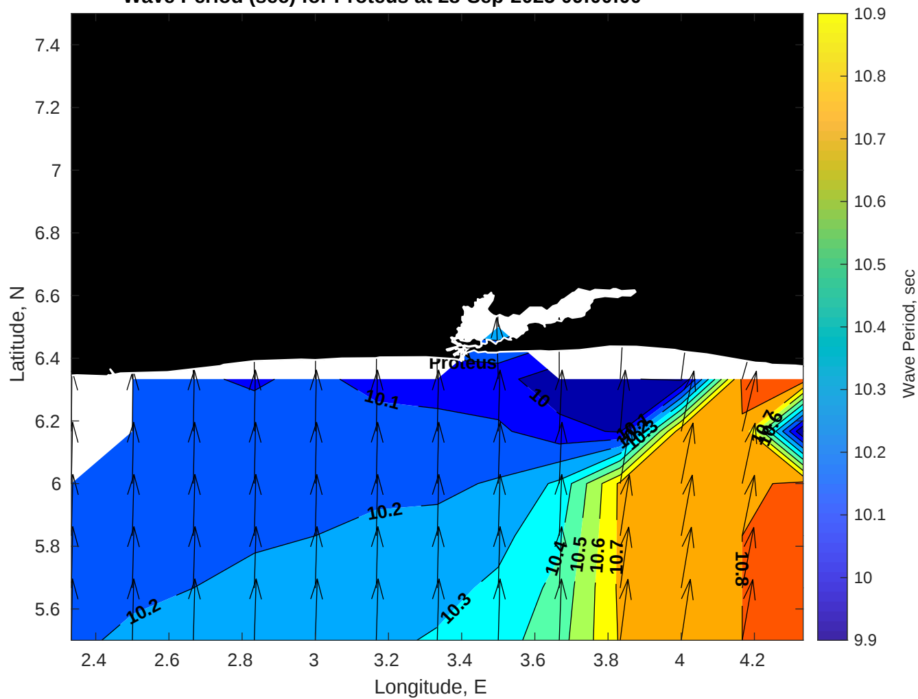
Wave Period (sec) for Proteus at 28-Sep-2025 09:00:00
