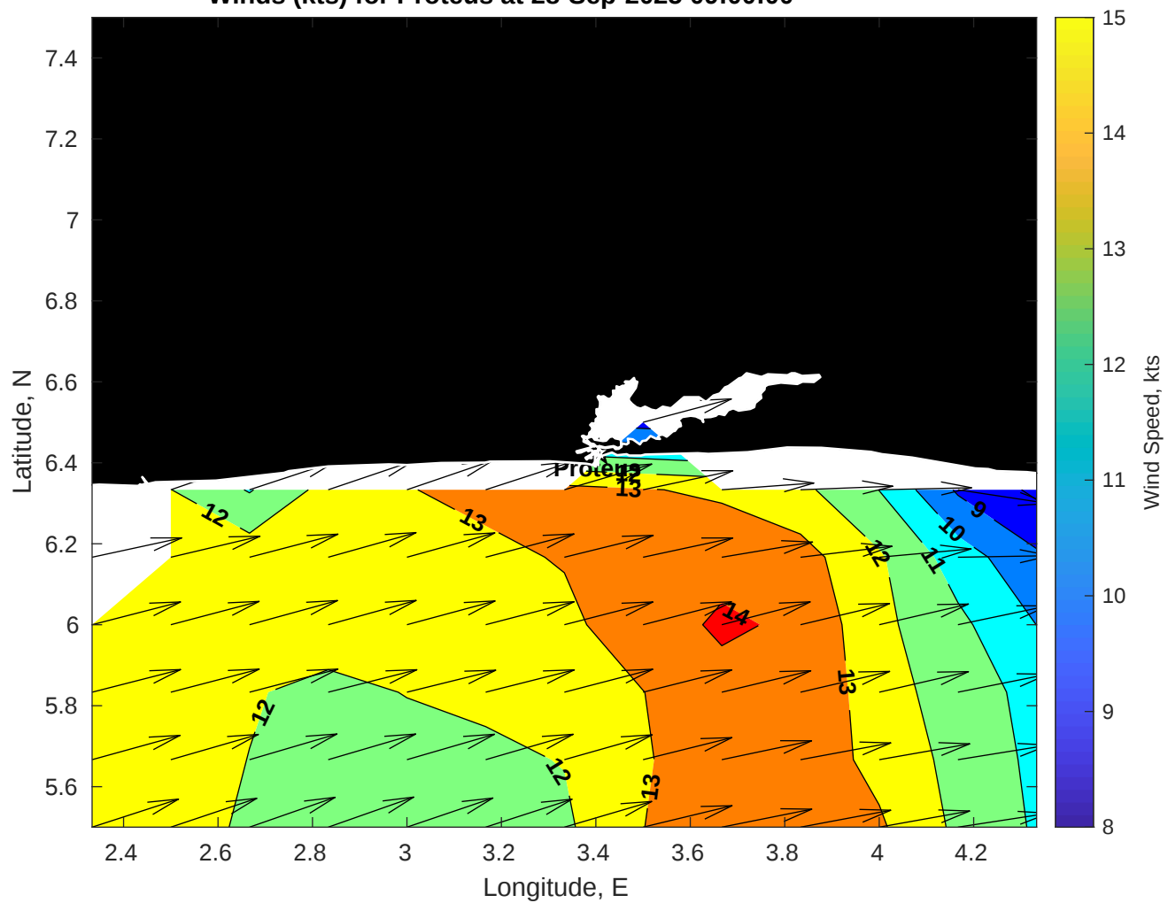
Winds (kts) for Proteus at 28-Sep-2025 09:00:00
