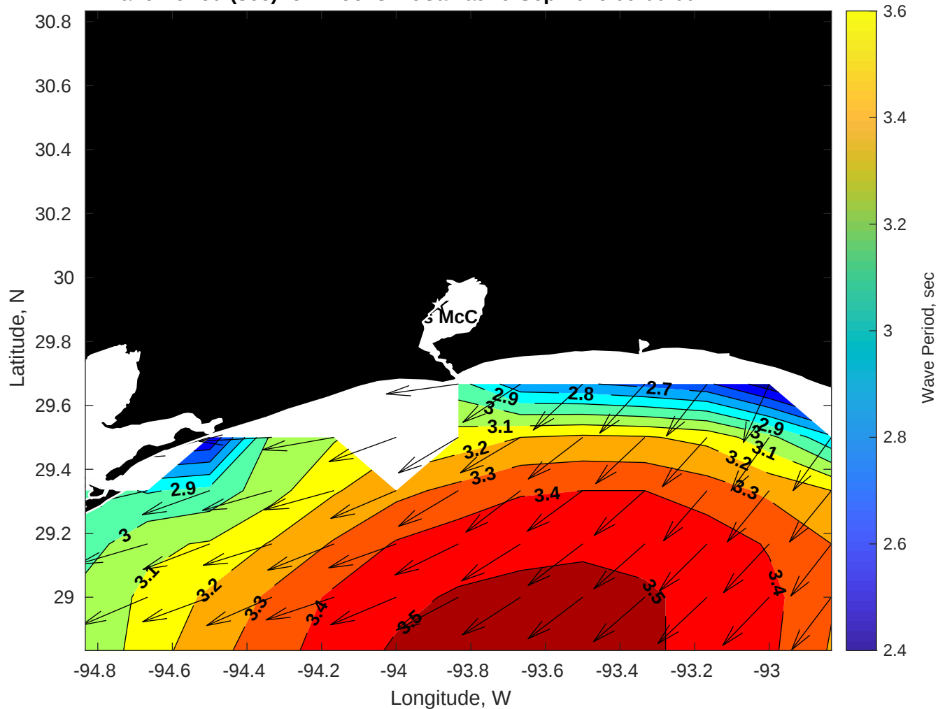
Wave Period (sec) for Brooks McCall at 29-Sep-2025 09:00:00
