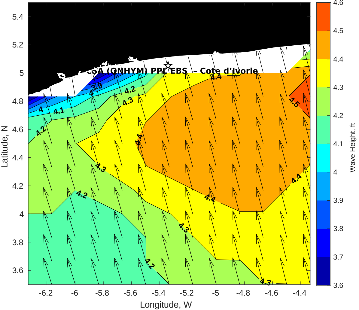
Wave Height (ft) for CSA (ONHYM) PPL EBS - Cote d'Ivoire at 29-Sep-2025 09:00:00
