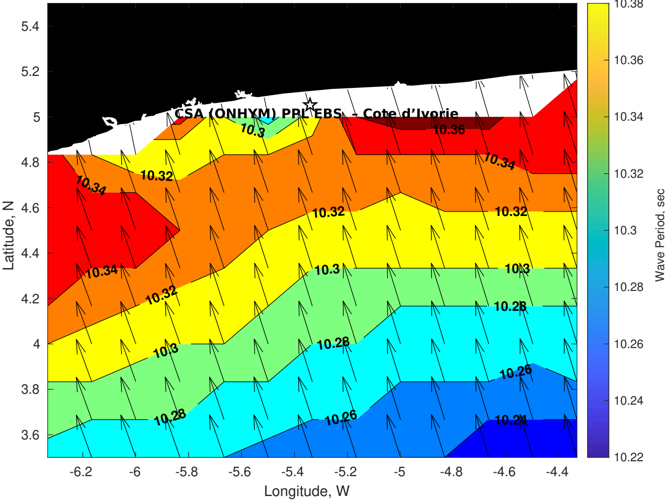
Wave Period (sec) for CSA (ONHYM) PPL EBS - Cote d'Ivoire at 29-Sep-2025 09:00:00
