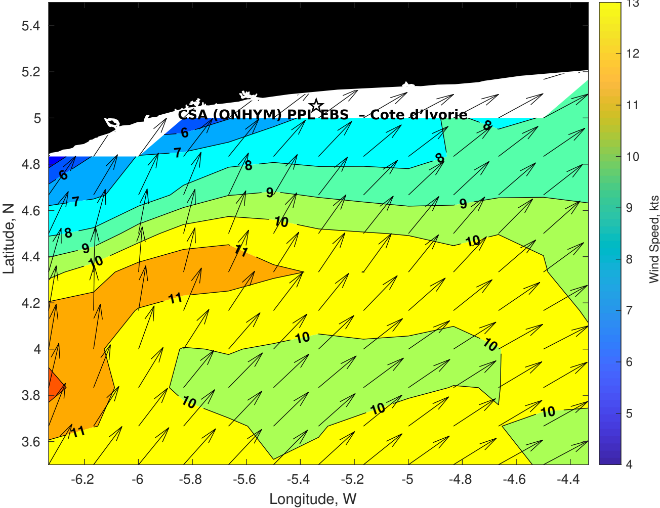
Winds (kts) for CSA (ONHYM) PPL EBS - Cote d'Ivoire at 29-Sep-2025 09:00:00
