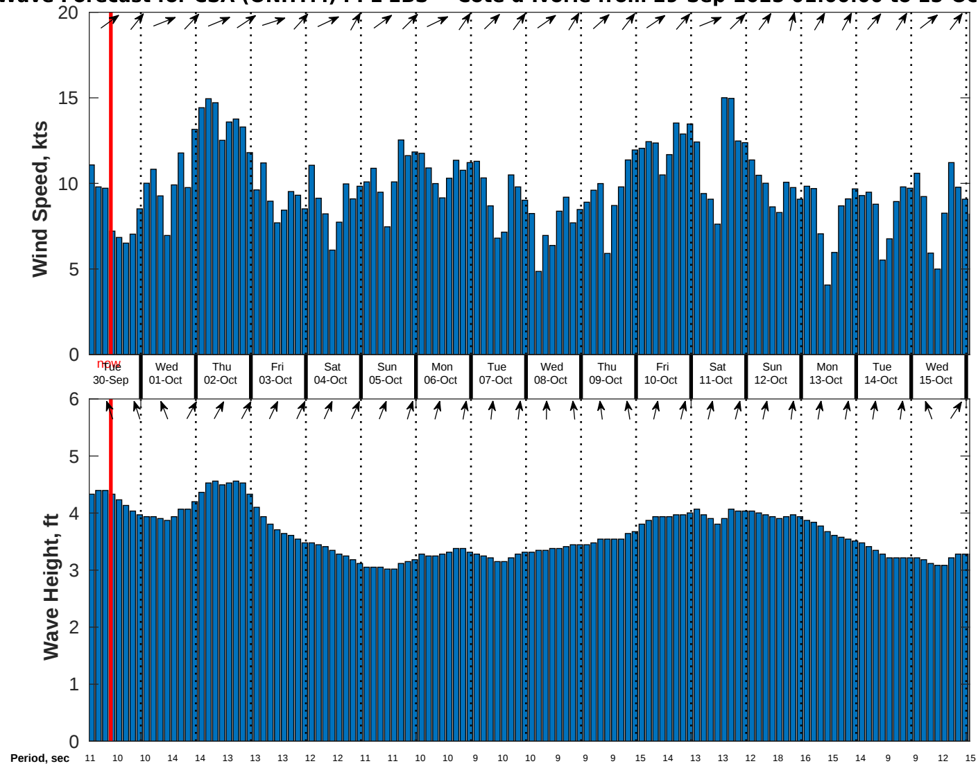
Wind & Wave Forecast for CSA (ONHYM) PPL EBS - Cote d'Ivoire from 29-Sep-2025 01:00:00 to 15-Oct-2025 01:00:00
