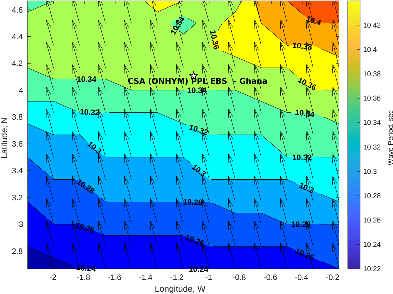
Wave Period (sec) for CSA (ONHYM) PPL EBS - Ghana at 29-Sep-2025 09:00:00
