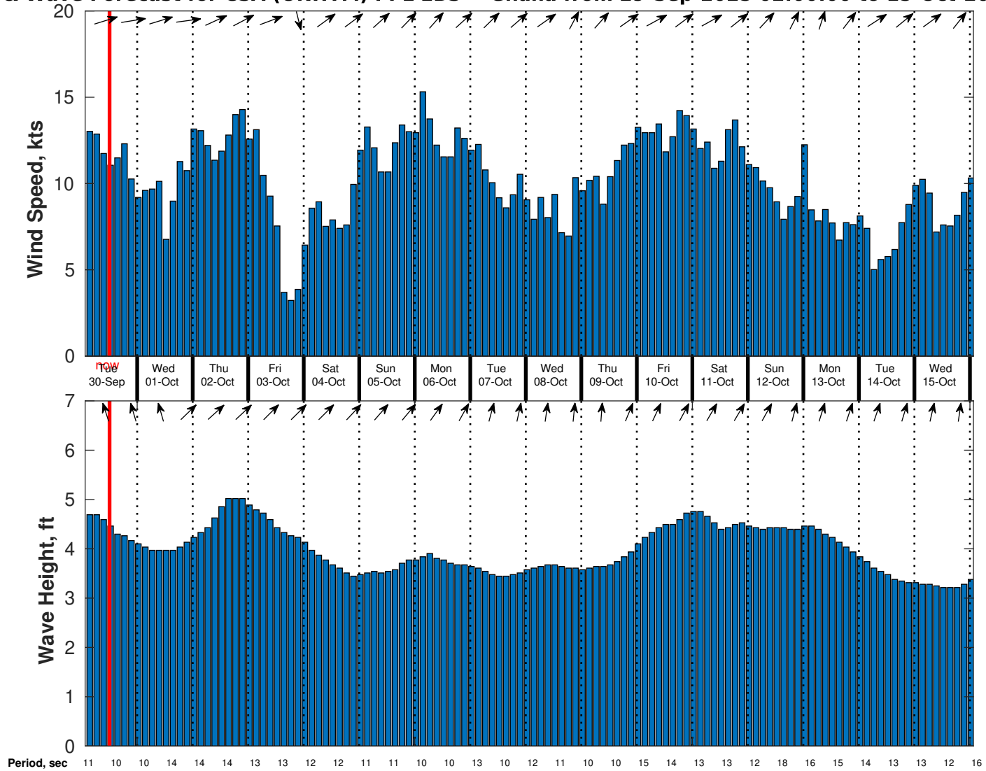
Wind & Wave Forecast for CSA (ONHYM) PPL EBS - Ghana from 29-Sep-2025 02:00:00 to 15-Oct-2025 02:00:00
