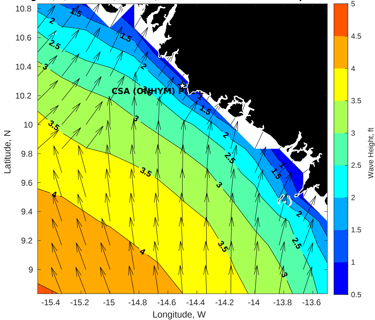
Wave Height (ft) for CSA (ONHYM) PPL EBS - Guinea at 29-Sep-2025 09:00:00
