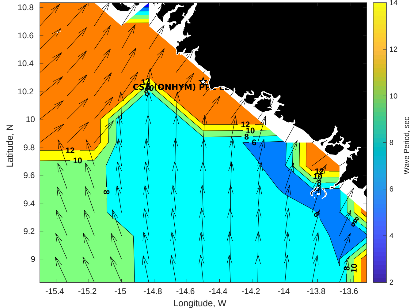
Wave Period (sec) for CSA (ONHYM) PPL EBS - Guinea at 29-Sep-2025 09:00:00
