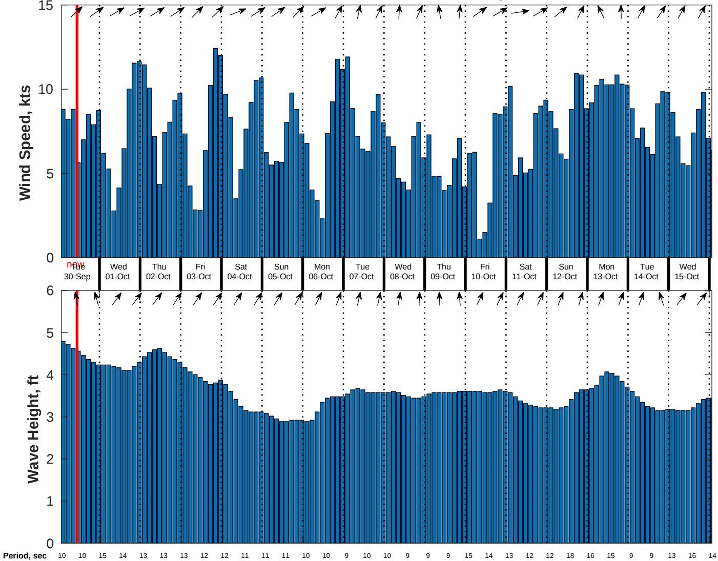
Wind & Wave Forecast for CSA (ONHYM) PPL EBS - Liberia from 29-Sep-2025 01:00:00 to 15-Oct-2025 01:00:00
