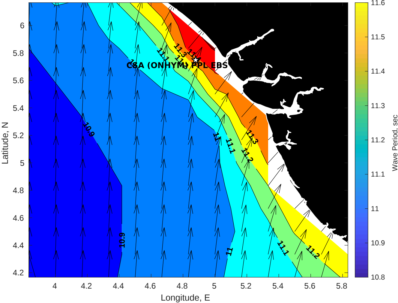
Wave Period (sec) for CSA (ONHYM) PPL EBS - Nigeria at 29-Sep-2025 09:00:00
