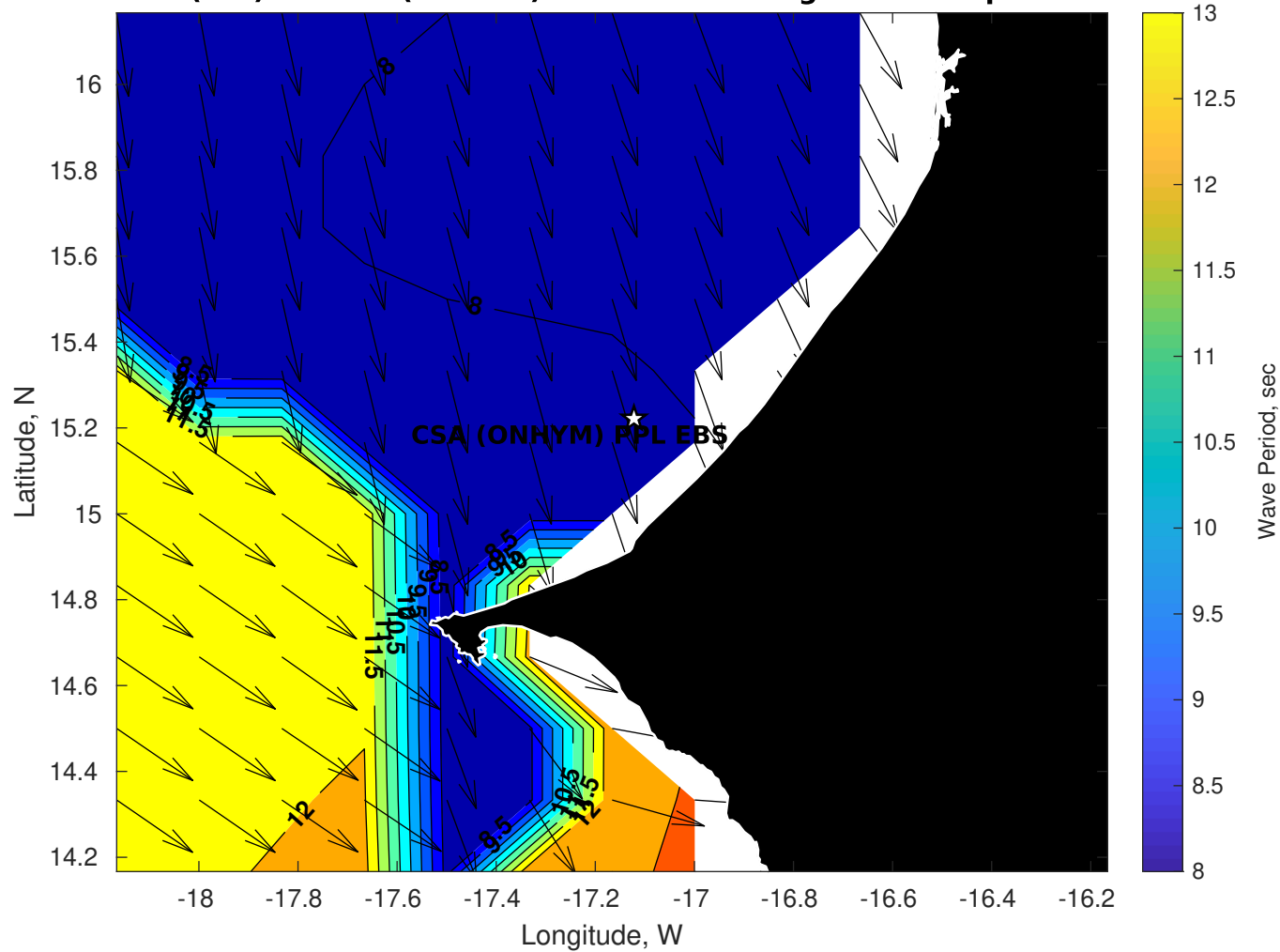
Wave Period (sec) for CSA (ONHYM) PPL EBS - Senegal at 29-Sep-2025 09:00:00
