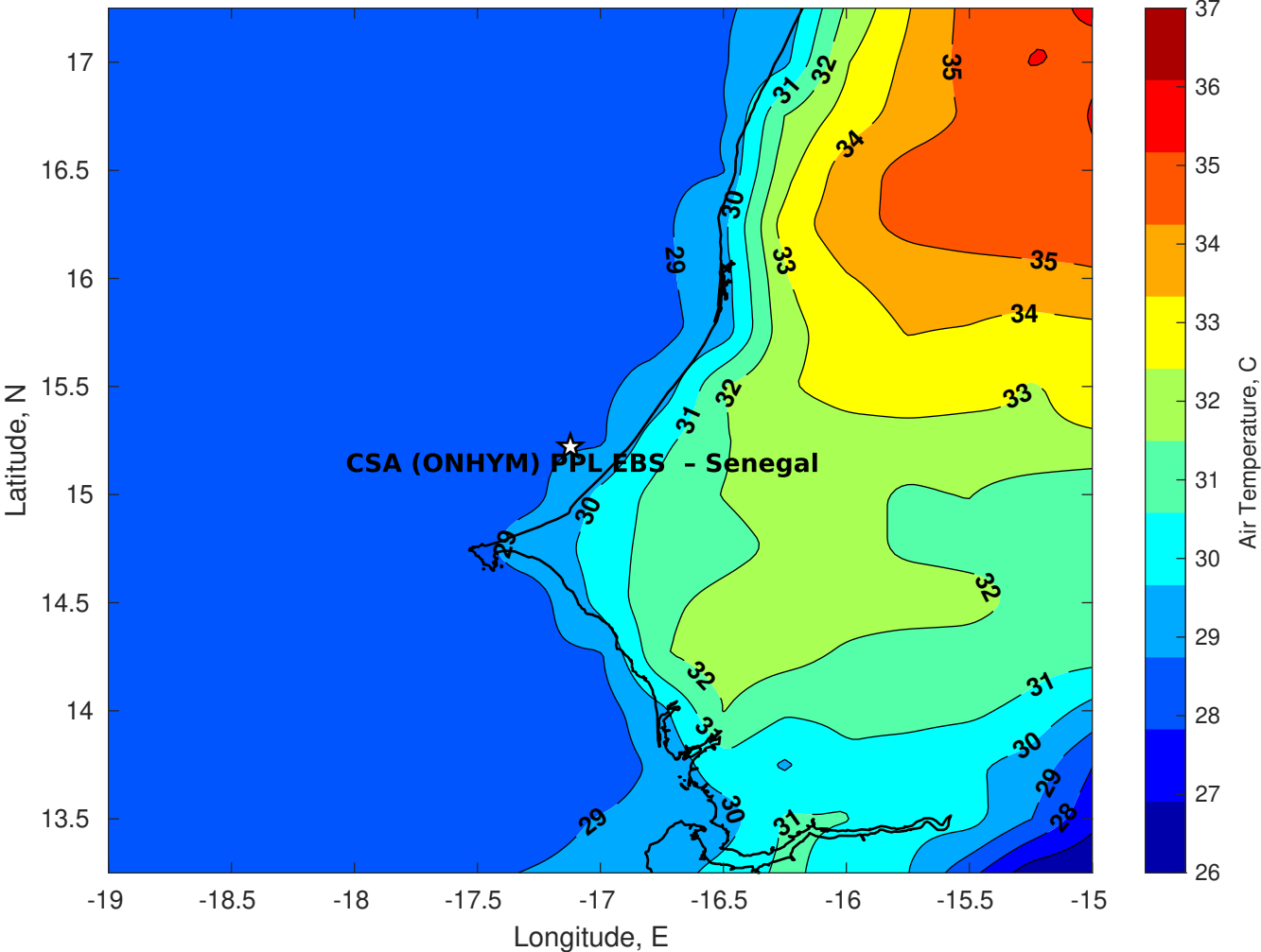
Air Temperature (C) for CSA (ONHYM) PPL EBS - Senegal at 17-Sep-2025
