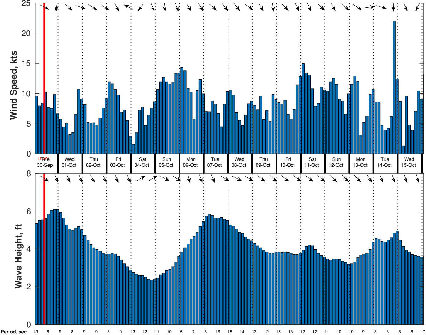
Wind & Wave Forecast for CSA (ONHYM) PPL EBS - Senegal from 29-Sep-2025 01:00:00 to 15-Oct-2025 01:00:00
