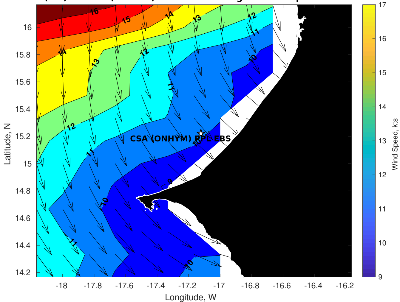
Winds (kts) for CSA (ONHYM) PPL EBS - Senegal at 29-Sep-2025 09:00:00
