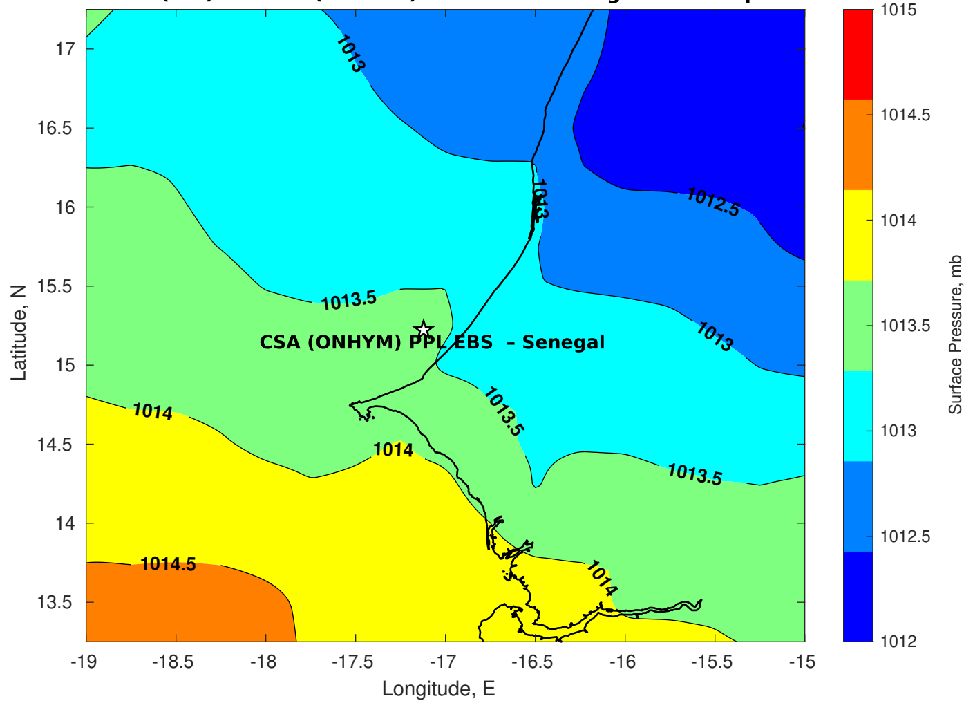
Surface Pressure (mb) for CSA (ONHYM) PPL EBS - Senegal at 19-Sep-2025 12:00:00
