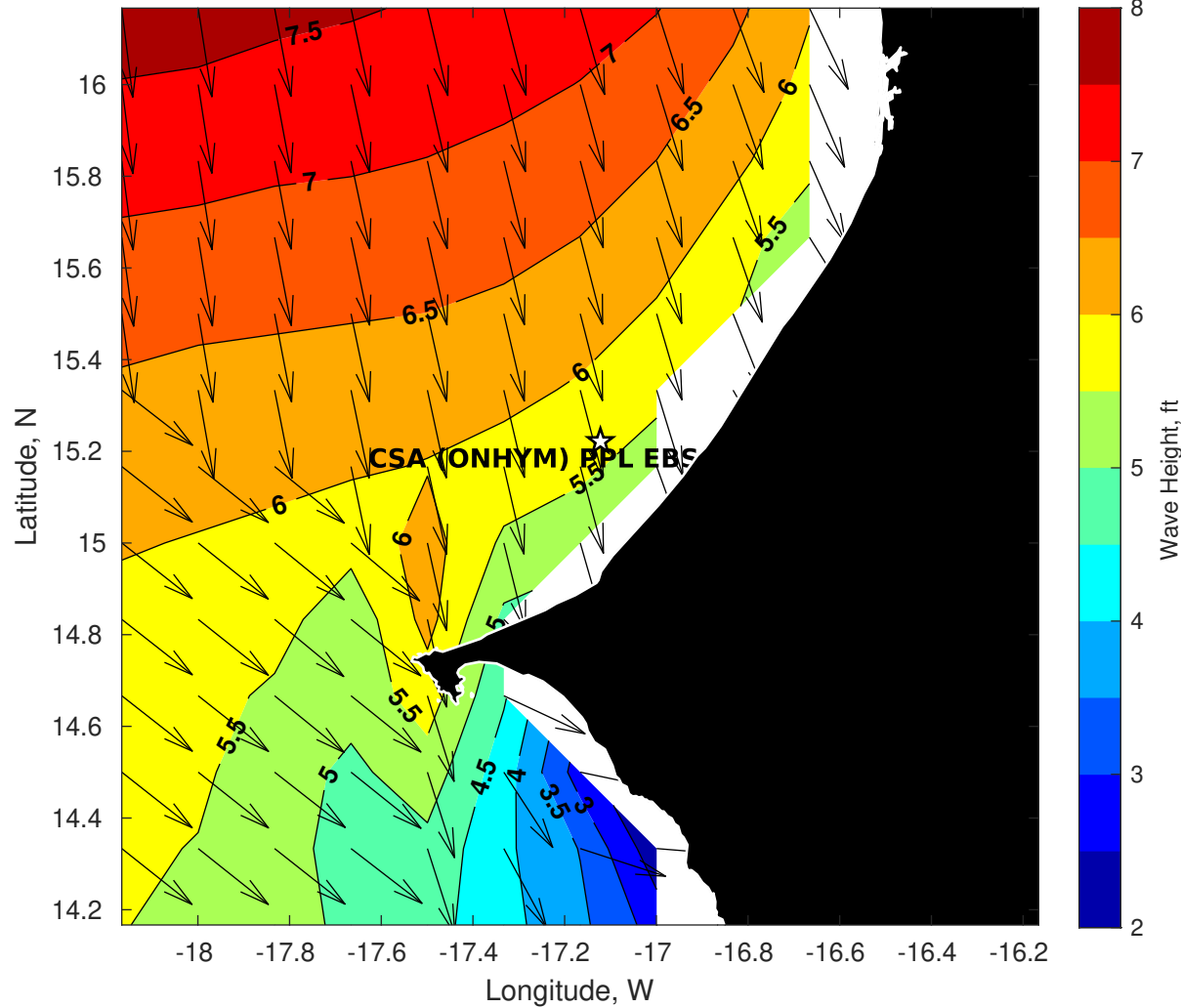
Wave Height (ft) for CSA (ONHYM) PPL EBS - Senegal at 29-Sep-2025 09:00:00
