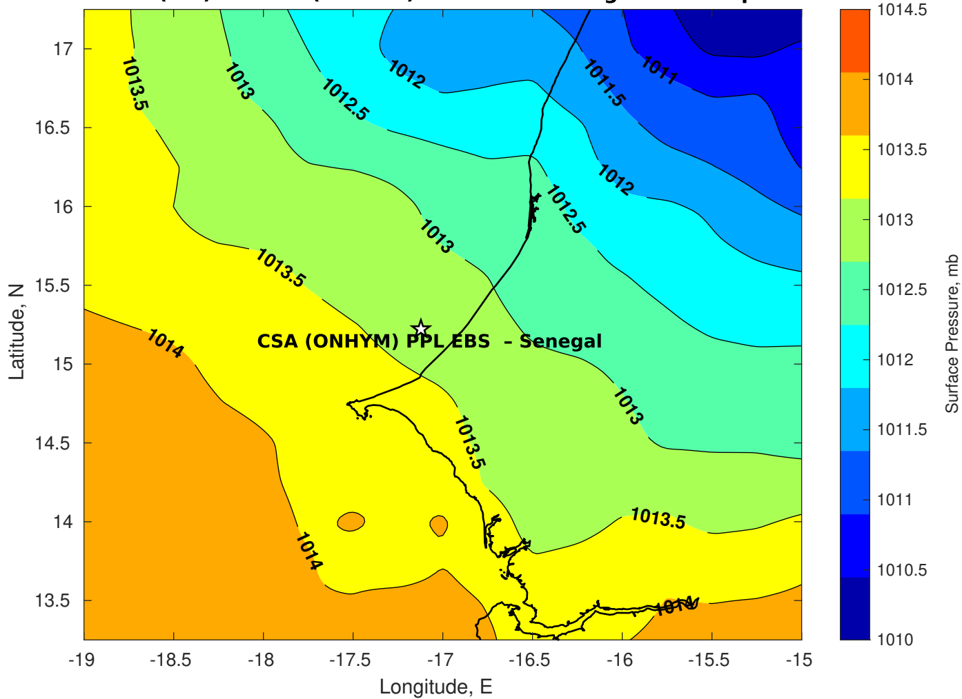
Surface Pressure (mb) for CSA (ONHYM) PPL EBS - Senegal at 18-Sep-2025 12:00:00
