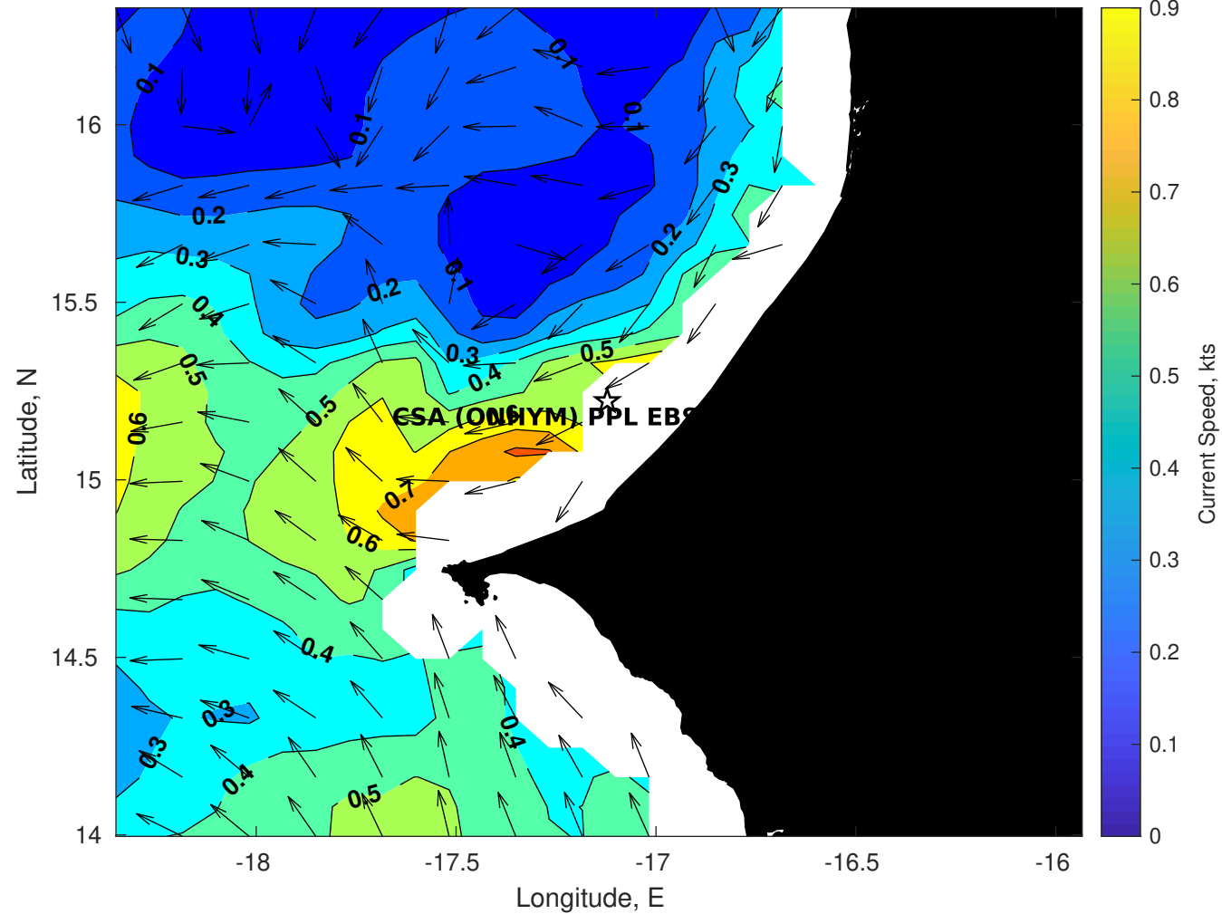
Surface Currents for CSA (ONHYM) PPL EBS - Senegal at 17-Sep-2025 00:00:00
