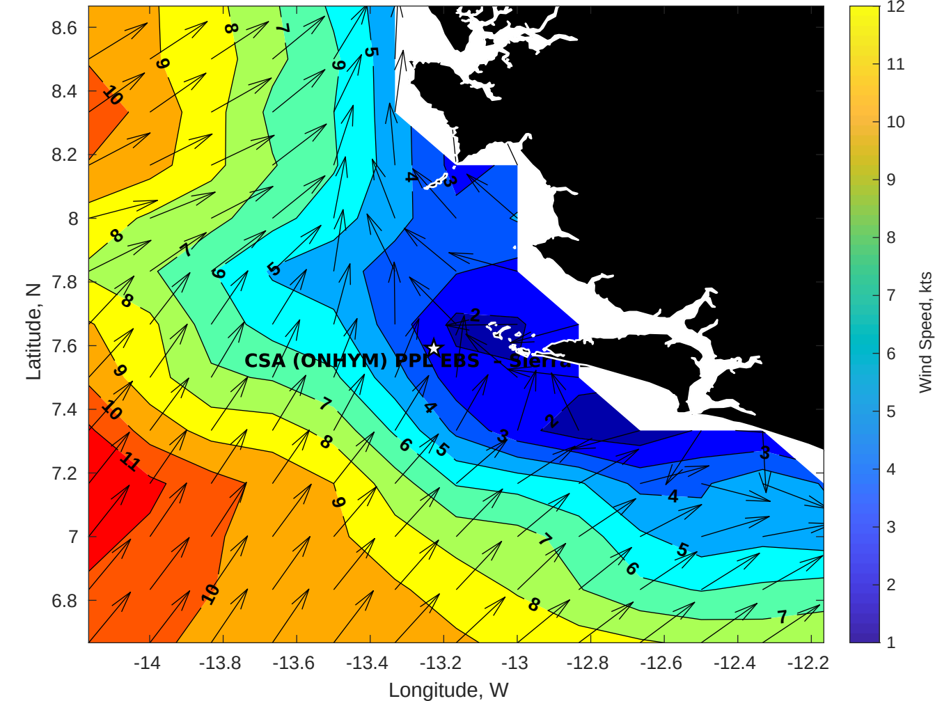
Winds (kts) for CSA (ONHYM) PPL EBS - Sierra Leone at 29-Sep-2025 09:00:00
