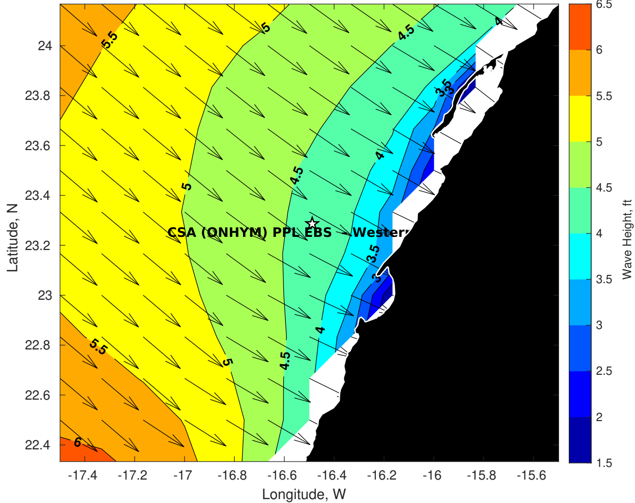
Wave Height (ft) for CSA (ONHYM) PPL EBS - Western Sahara at 29-Sep-2025 09:00:00
