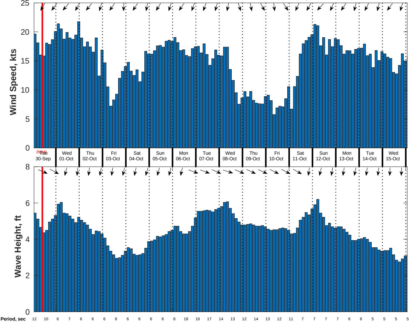
Wind & Wave Forecast for CSA (ONHYM) PPL EBS - Western Sahara from 29-Sep-2025 01:00:00 to 15-Oct-2025 01:00:00
