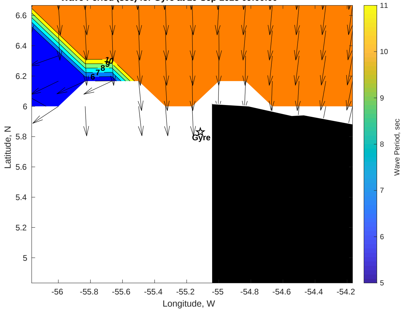
Wave Period (sec) for Gyre at 29-Sep-2025 09:00:00
