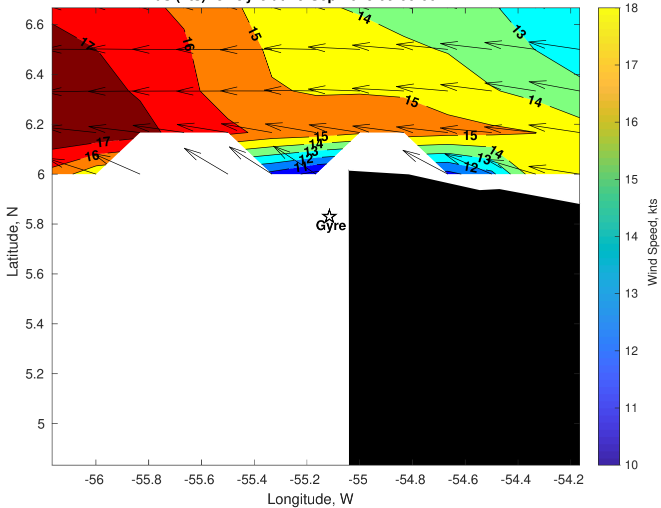
Winds (kts) for Gyre at 29-Sep-2025 09:00:00
