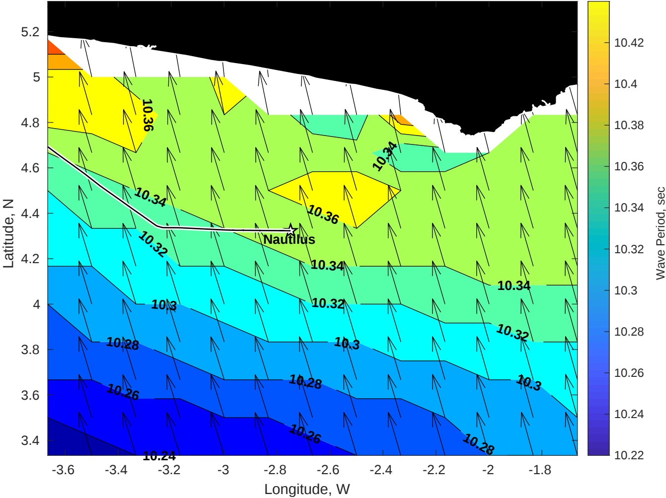
Wave Period (sec) for Nautilus at 29-Sep-2025 09:00:00
