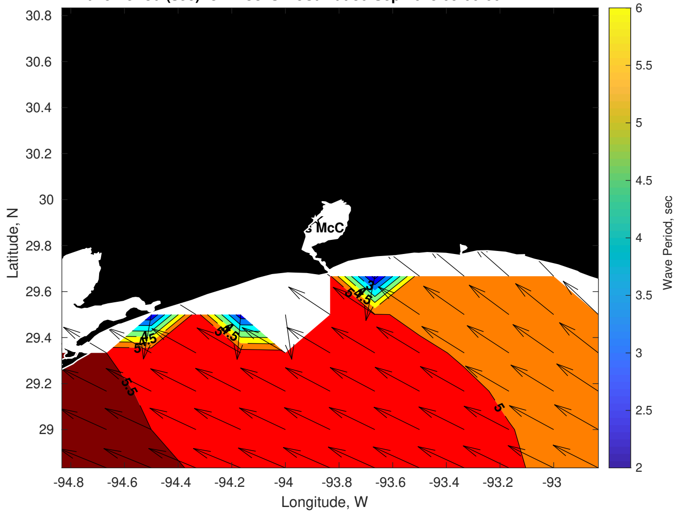
Wave Period (sec) for Brooks McCall at 30-Sep-2025 09:00:00
