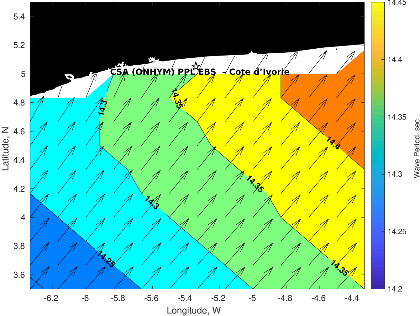
Wave Period (sec) for CSA (ONHYM) PPL EBS - Cote d'Ivoire at 30-Sep-2025 09:00:00
