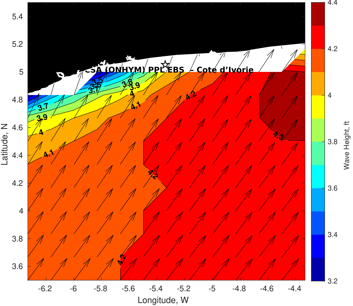
Wave Height (ft) for CSA (ONHYM) PPL EBS - Cote d'Ivoire at 30-Sep-2025 09:00:00
