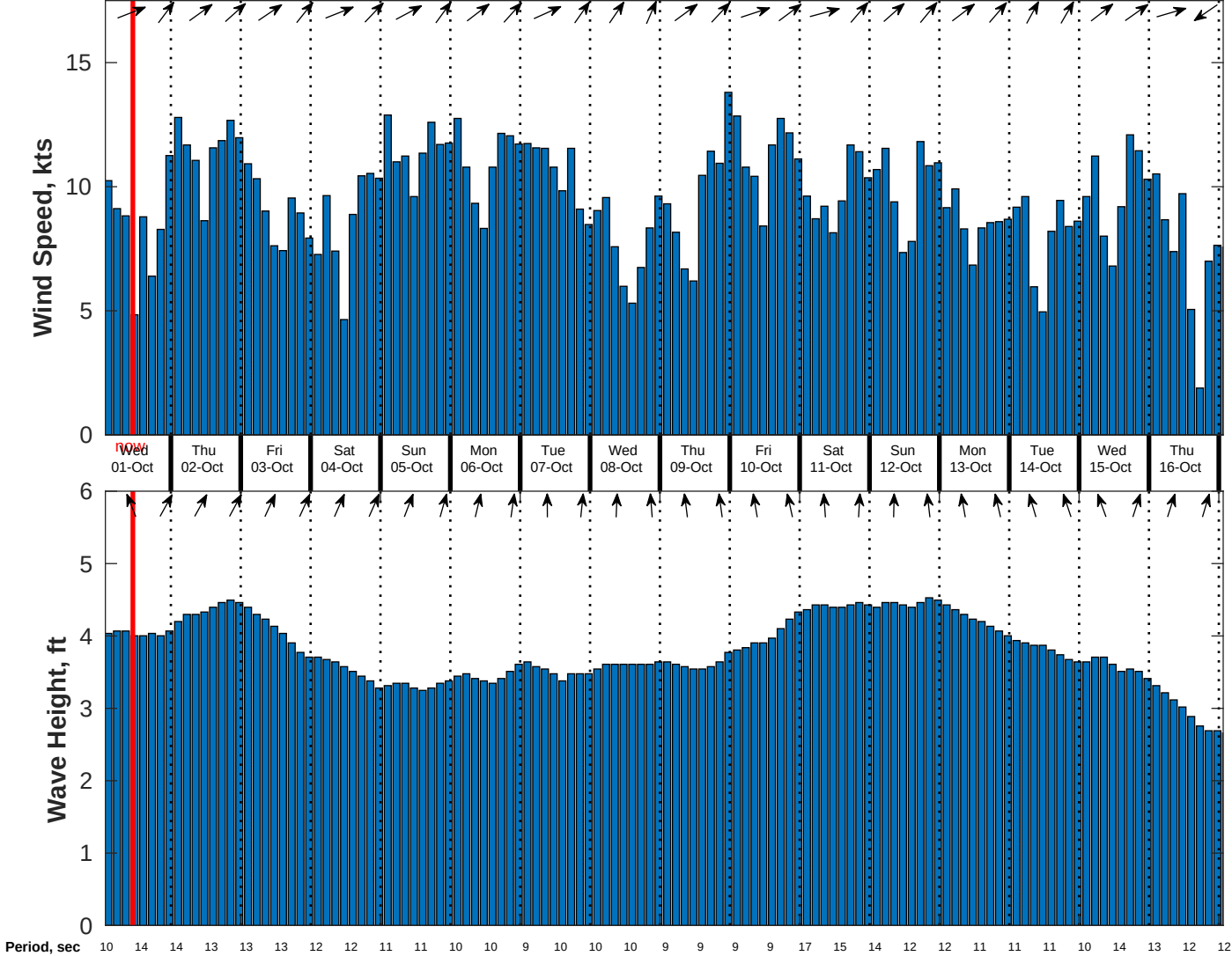
Wind & Wave Forecast for CSA (ONHYM) PPL EBS - Cote d'Ivoire from 30-Sep-2025 01:00:00 to 16-Oct-2025 01:00:00
