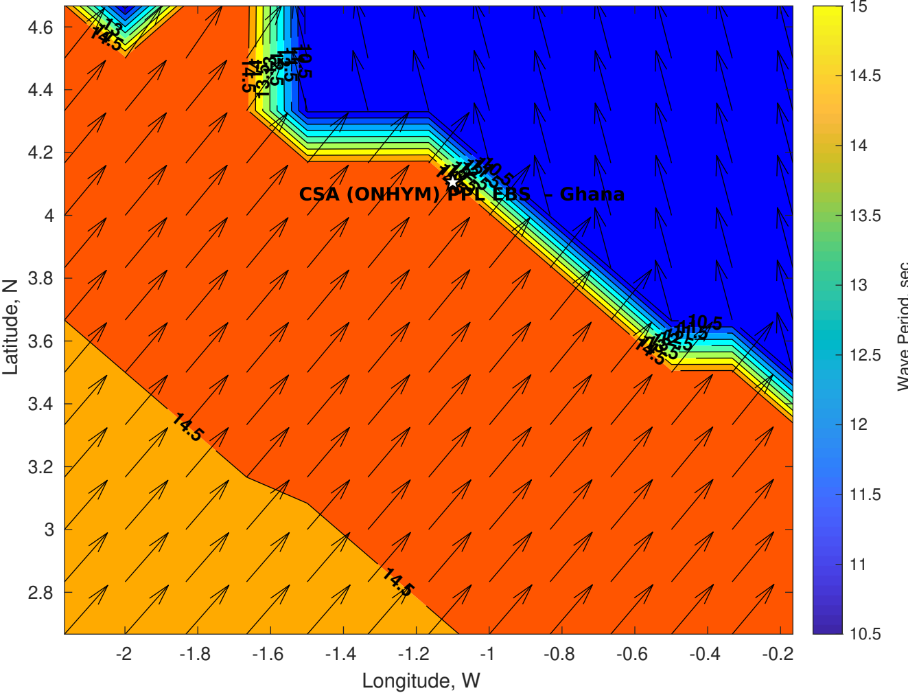
Wave Period (sec) for CSA (ONHYM) PPL EBS - Ghana at 30-Sep-2025 09:00:00
