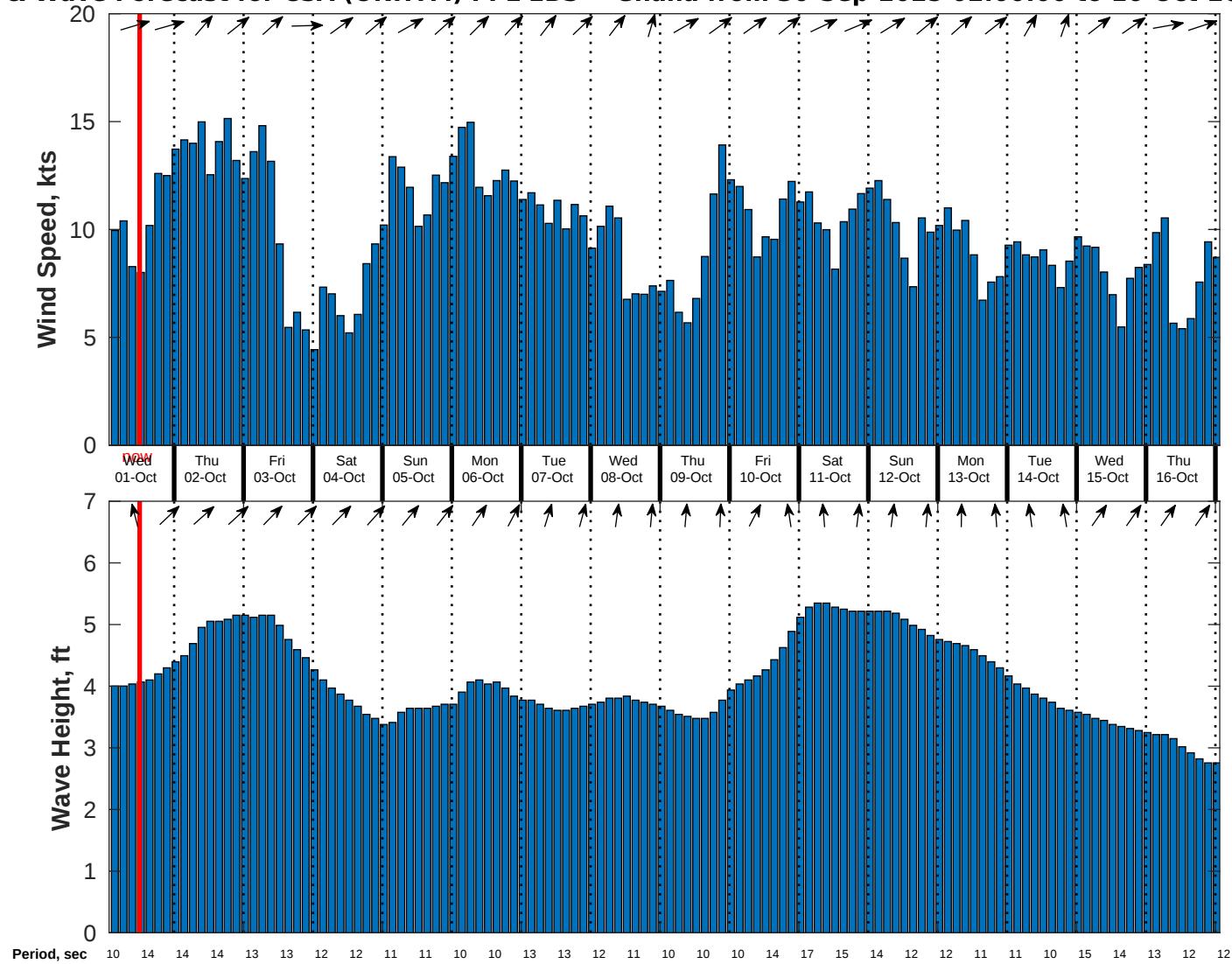
Wind & Wave Forecast for CSA (ONHYM) PPL EBS - Ghana from 30-Sep-2025 02:00:00 to 16-Oct-2025 02:00:00
