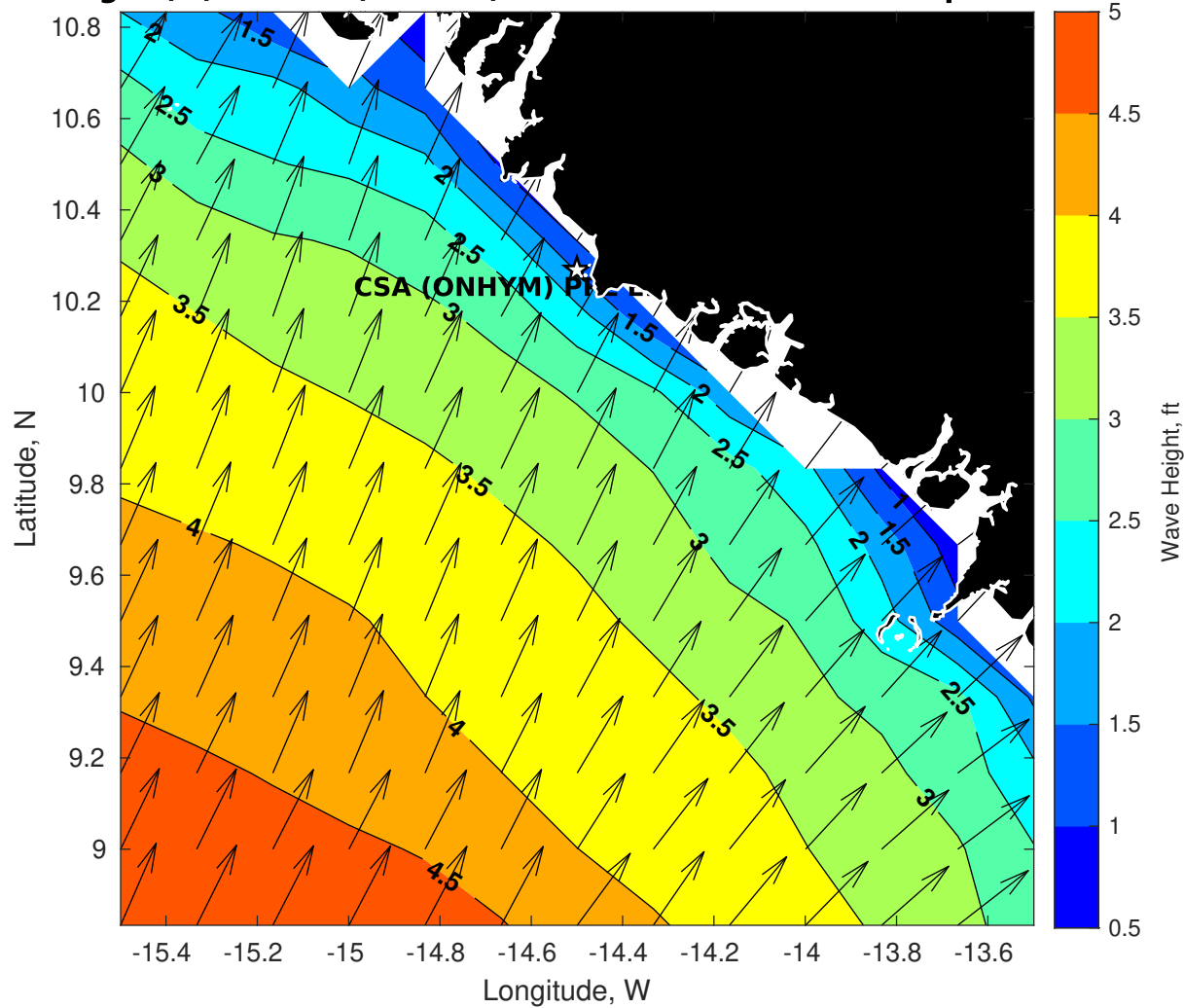
Wave Height (ft) for CSA (ONHYM) PPL EBS - Guinea at 30-Sep-2025 09:00:00
