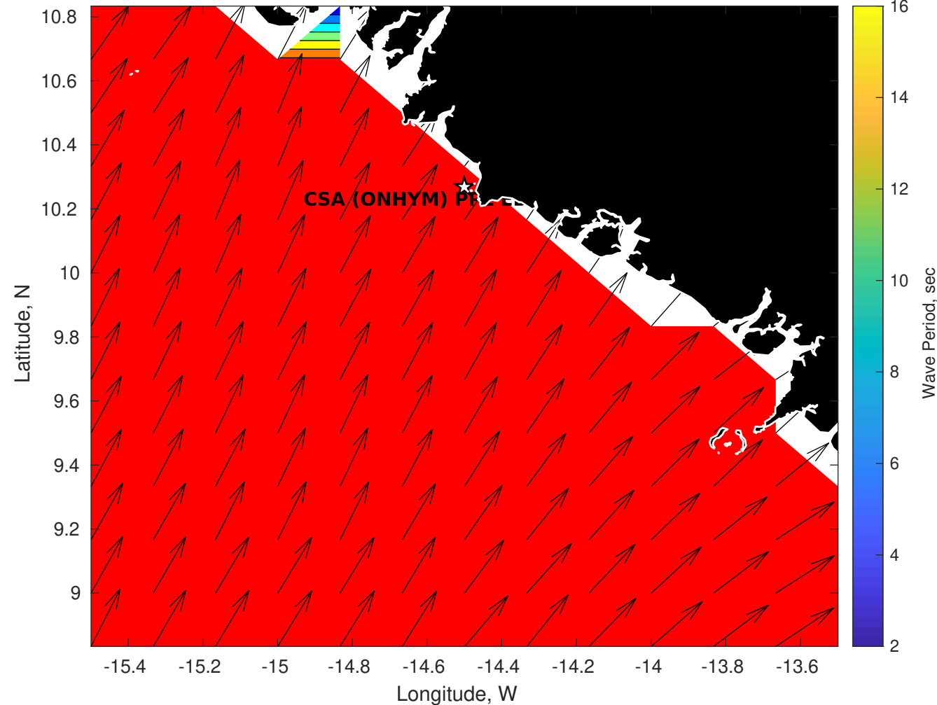
Wave Period (sec) for CSA (ONHYM) PPL EBS - Guinea at 30-Sep-2025 09:00:00
