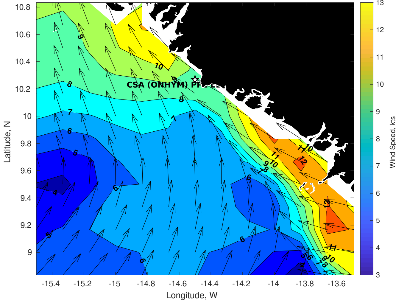
Winds (kts) for CSA (ONHYM) PPL EBS - Guinea at 30-Sep-2025 09:00:00
