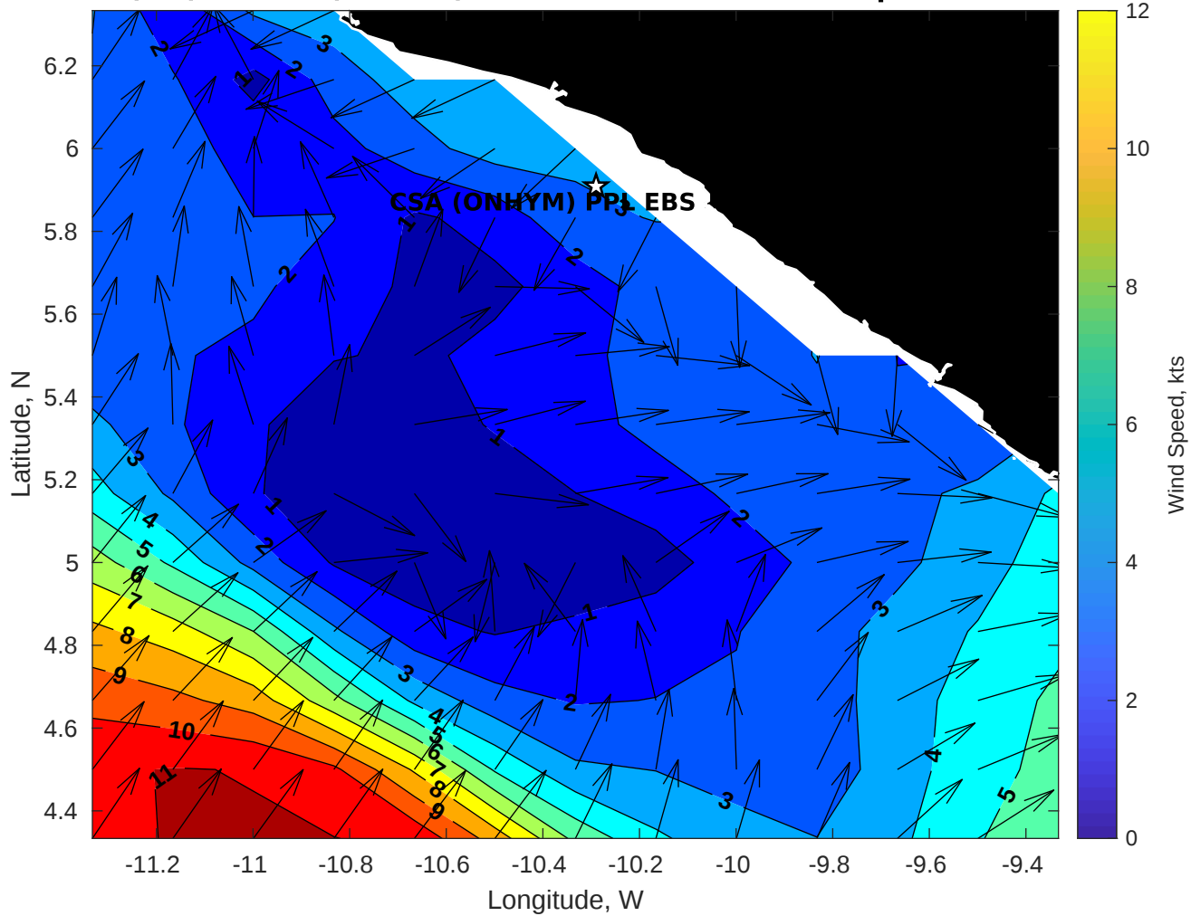
Winds (kts) for CSA (ONHYM) PPL EBS - Liberia at 30-Sep-2025 09:00:00
