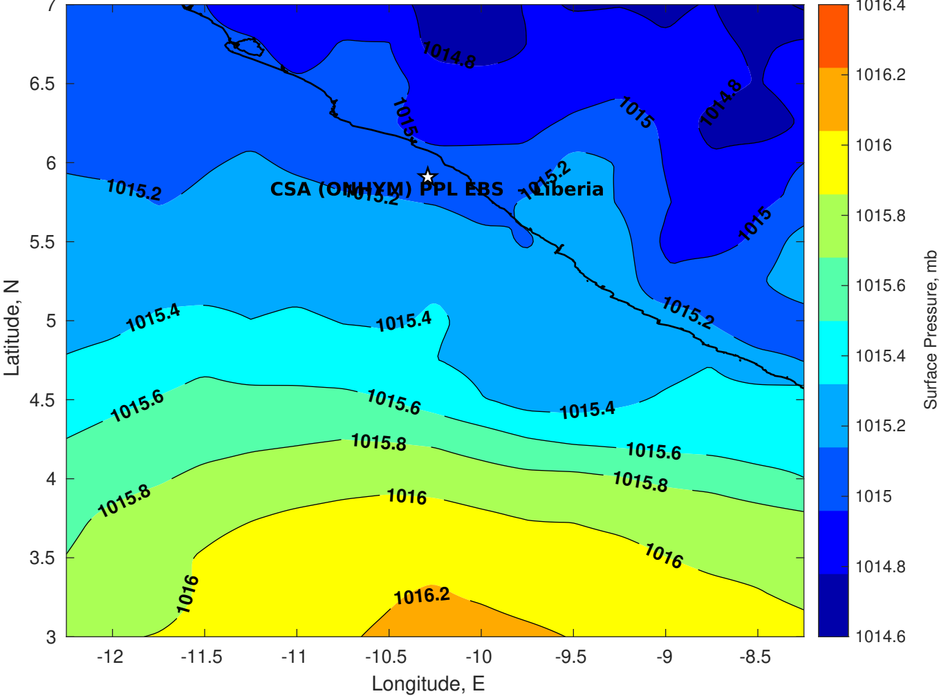
Surface Pressure (mb) for CSA (ONHYM) PPL EBS - Liberia at 19-Sep-2025 12:00:00
