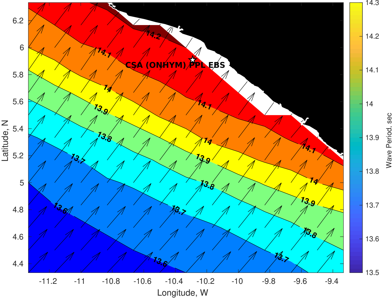
Wave Period (sec) for CSA (ONHYM) PPL EBS - Liberia at 30-Sep-2025 09:00:00
