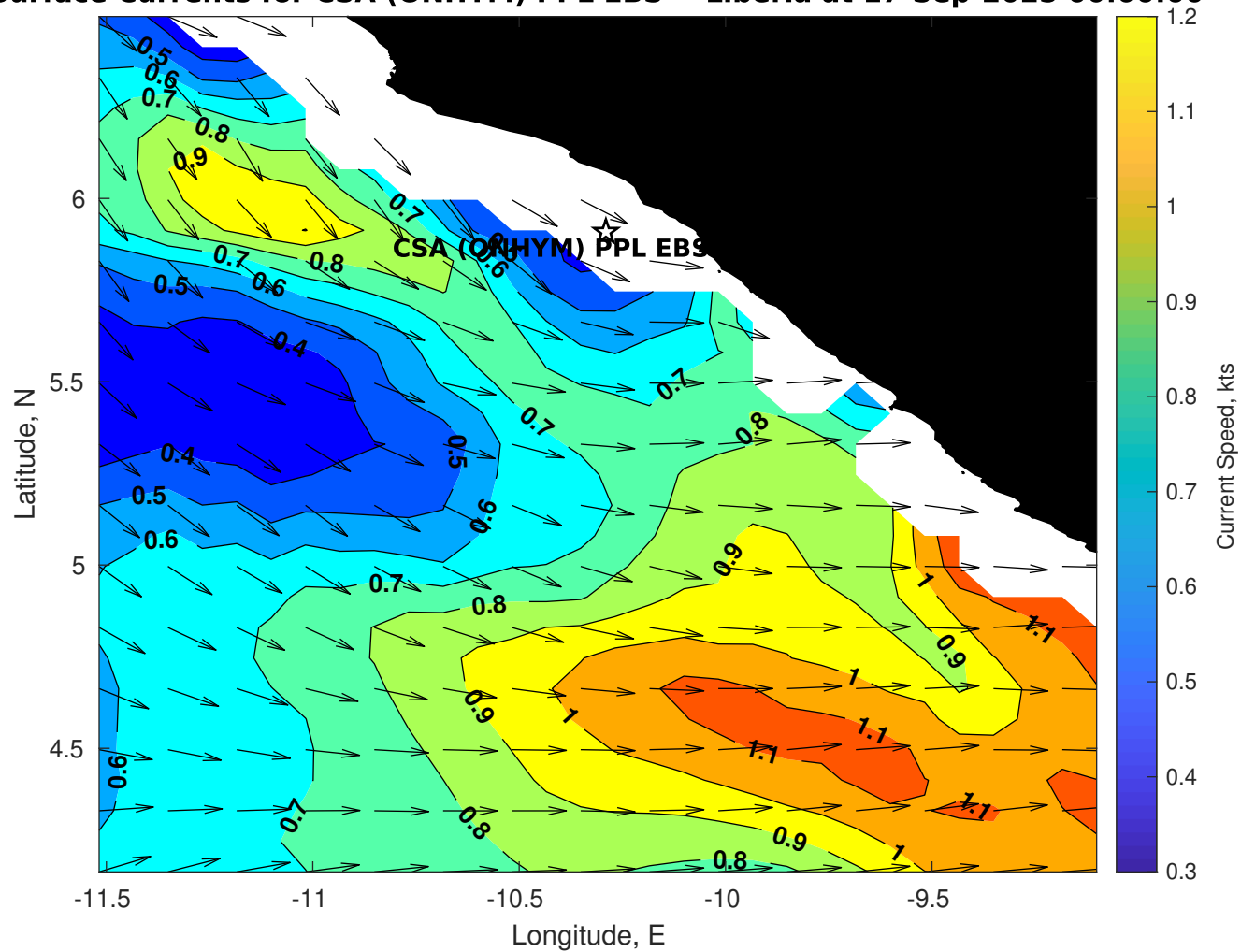
Surface Currents for CSA (ONHYM) PPL EBS - Liberia at 17-Sep-2025 00:00:00
