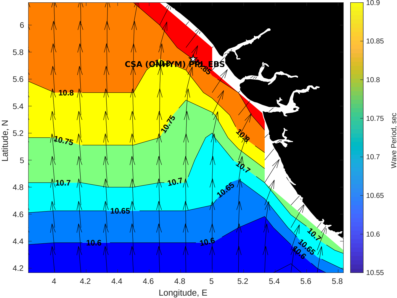
Wave Period (sec) for CSA (ONHYM) PPL EBS - Nigeria at 30-Sep-2025 09:00:00
