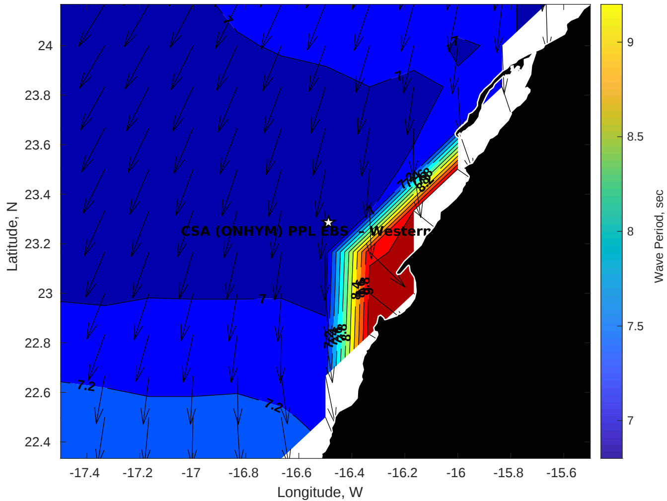
Wave Period (sec) for CSA (ONHYM) PPL EBS - Western Sahara at 30-Sep-2025 09:00:00
