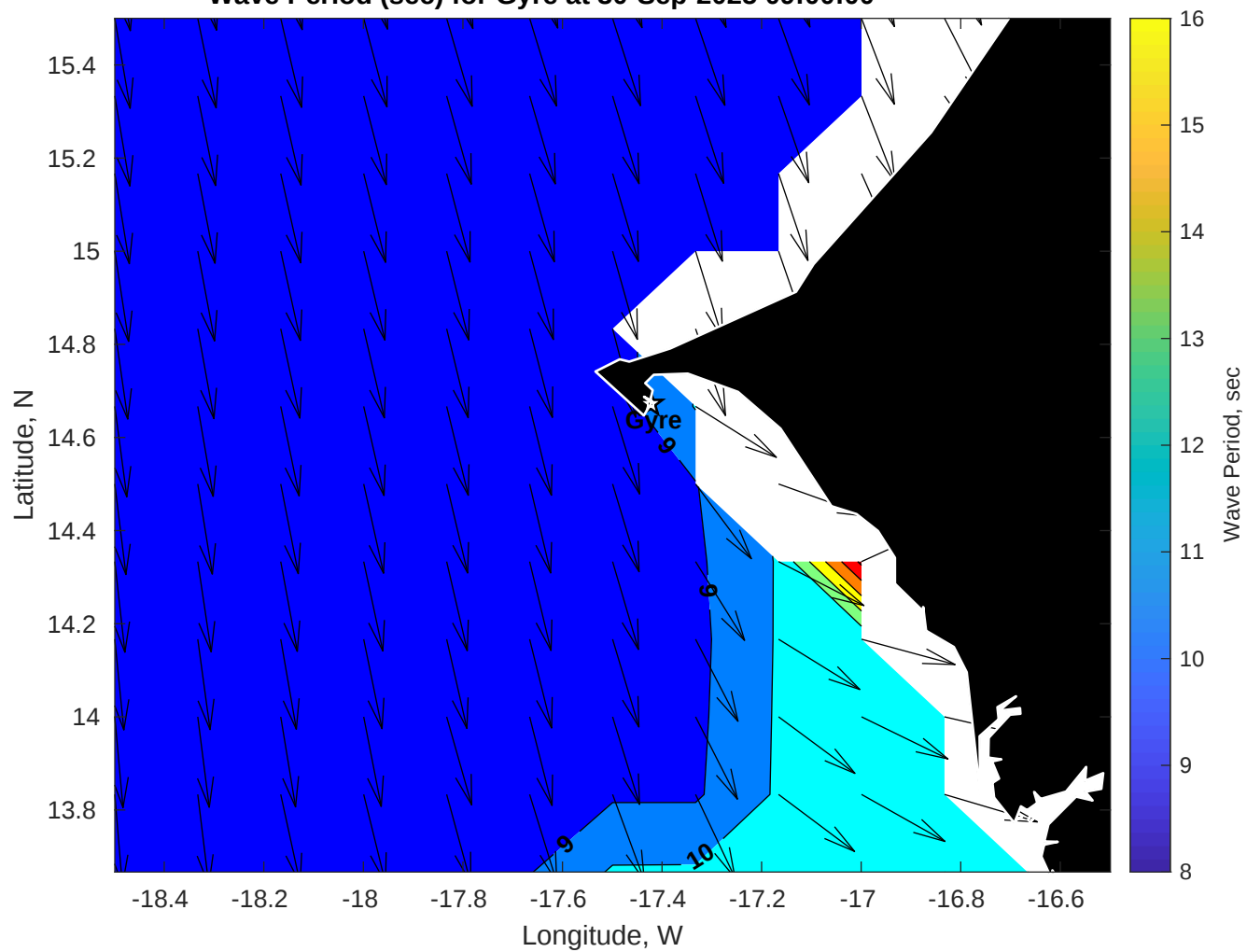
Wave Period (sec) for Gyre at 30-Sep-2025 09:00:00
