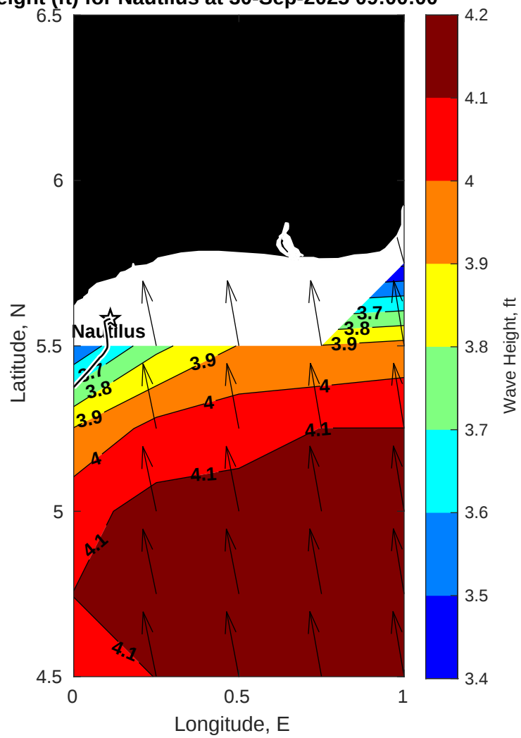
Wave Height (ft) for Nautilus at 30-Sep-2025 09:00:00
