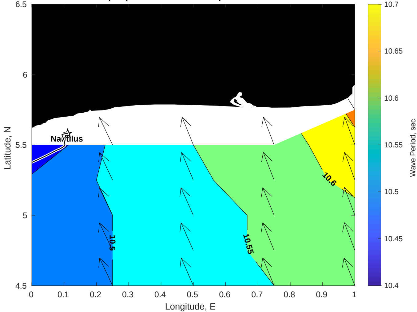
Wave Period (sec) for Nautilus at 30-Sep-2025 09:00:00
