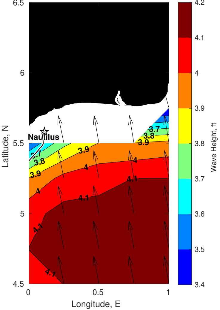
Wave Height (ft) for Nautilus at 30-Sep-2025 09:00:00
