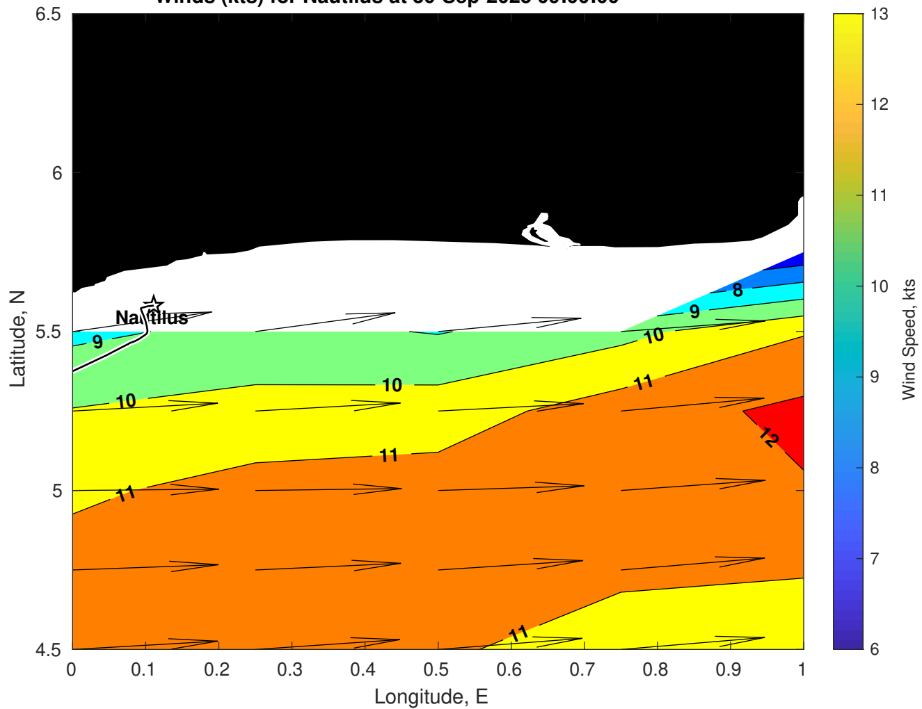
Winds (kts) for Nautilus at 30-Sep-2025 09:00:00
