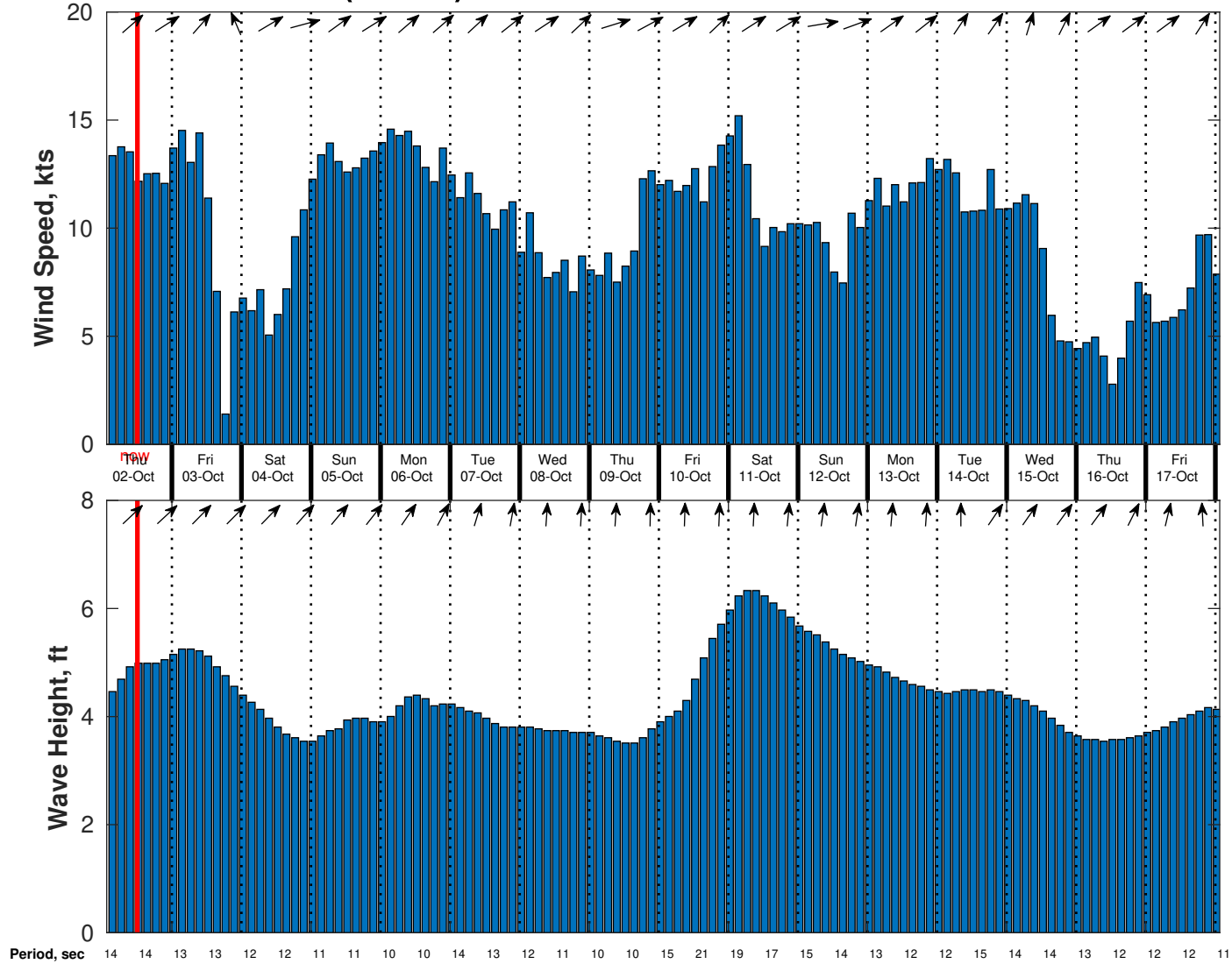
Wind & Wave Forecast for CSA (ONHYM) PPL EBS - Ghana from 01-Oct-2025 02:00:00 to 17-Oct-2025 02:00:00
