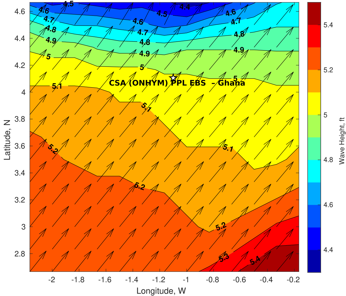
Wave Height (ft) for CSA (ONHYM) PPL EBS - Ghana at 01-Oct-2025 09:00:00
